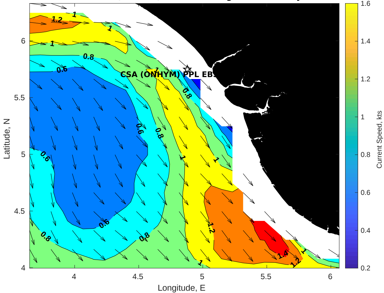
Surface Currents for CSA (ONHYM) PPL EBS - Nigeria at 19-May-2025 00:00:00
