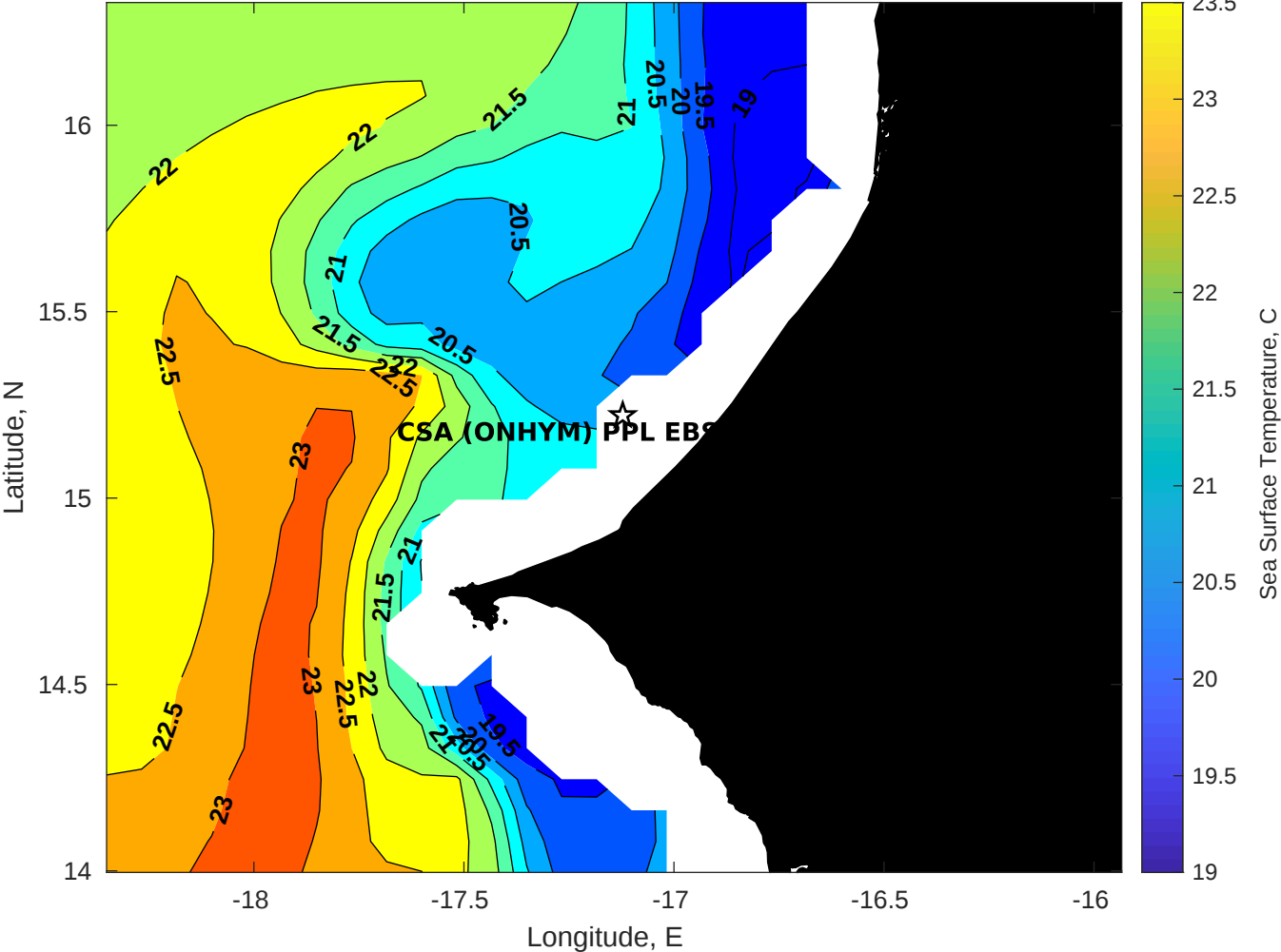
SST for CSA (ONHYM) PPL EBS - Senegal at 19-May-2025 00:00:00
