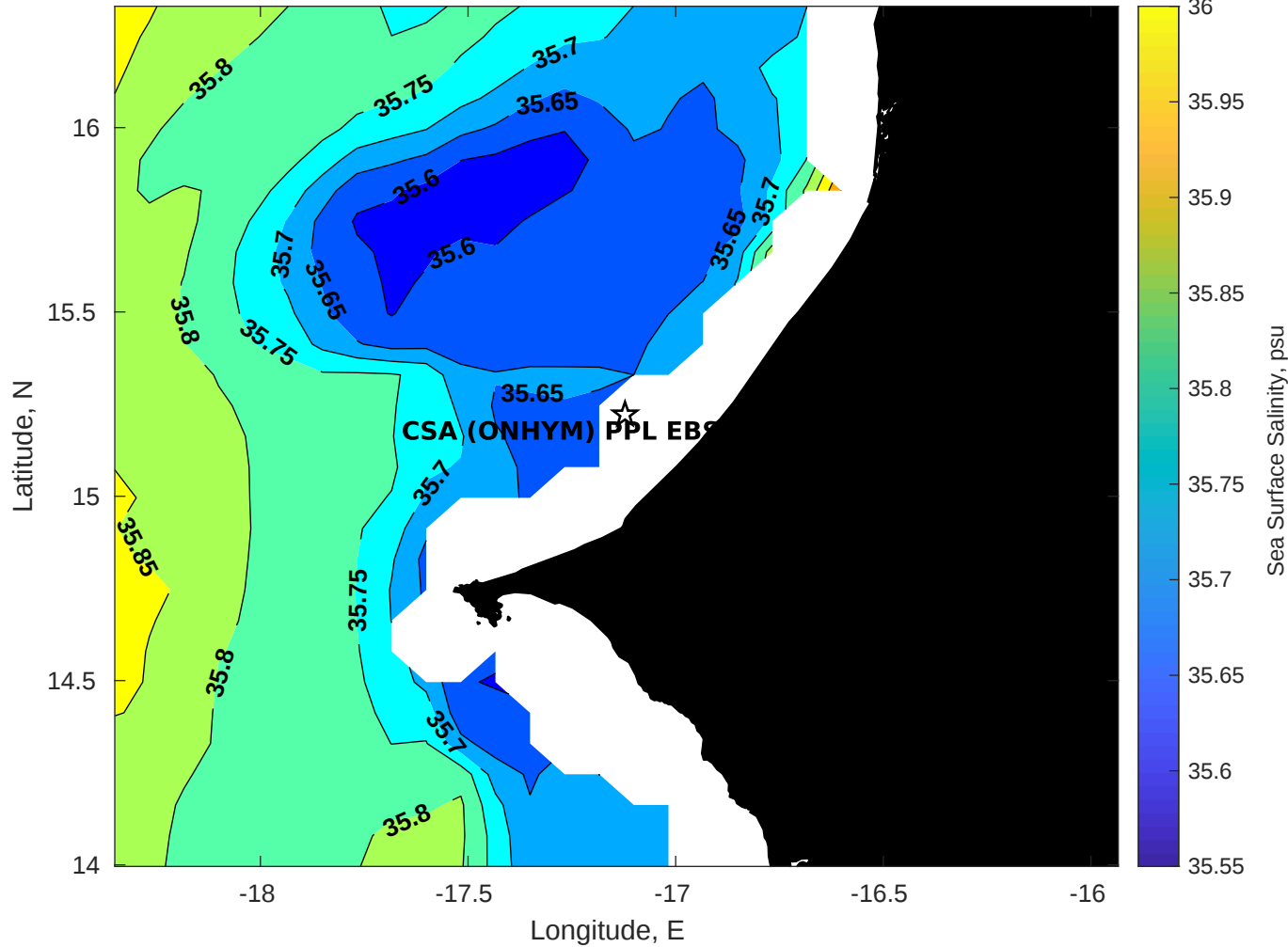
Surface Salinity for CSA (ONHYM) PPL EBS - Senegal at 19-May-2025 00:00:00
