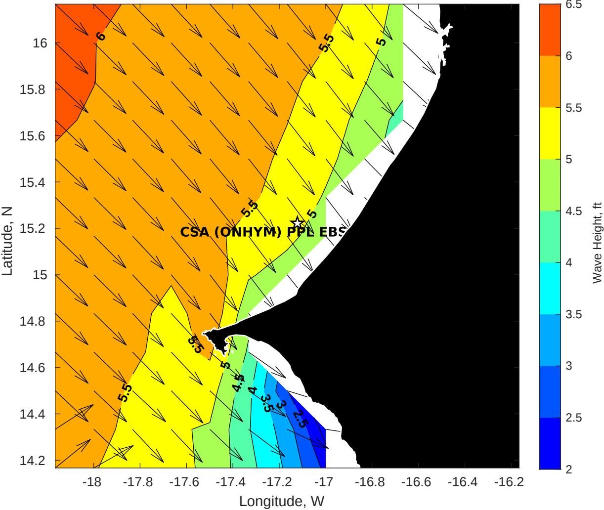
Wave Height (ft) for CSA (ONHYM) PPL EBS - Senegal at 20-May-2025 09:00:00
