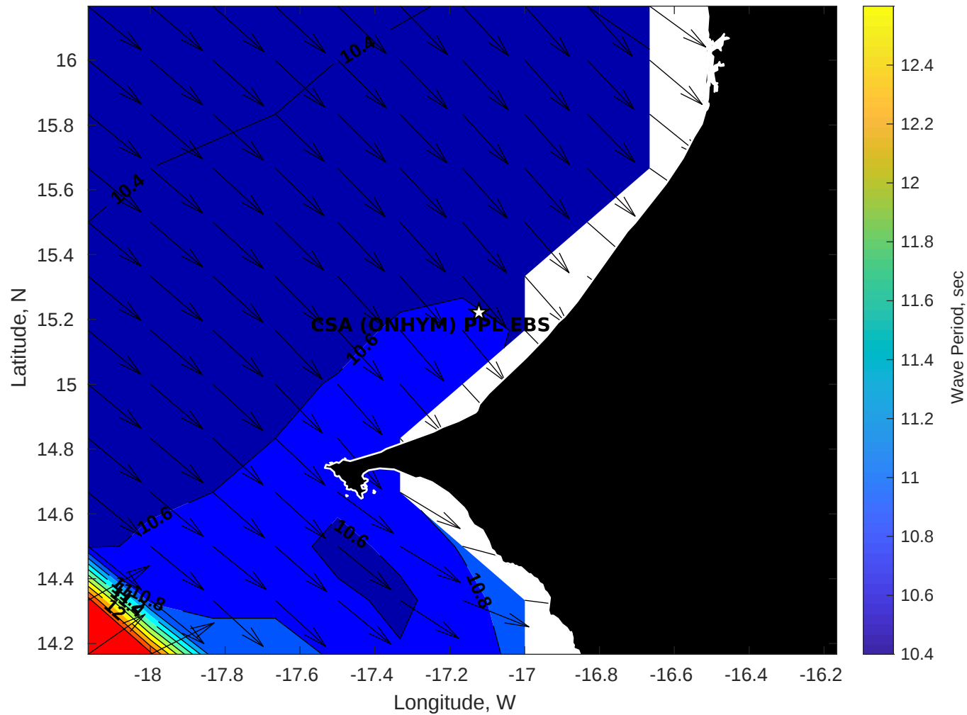
Wave Period (sec) for CSA (ONHYM) PPL EBS - Senegal at 20-May-2025 09:00:00
