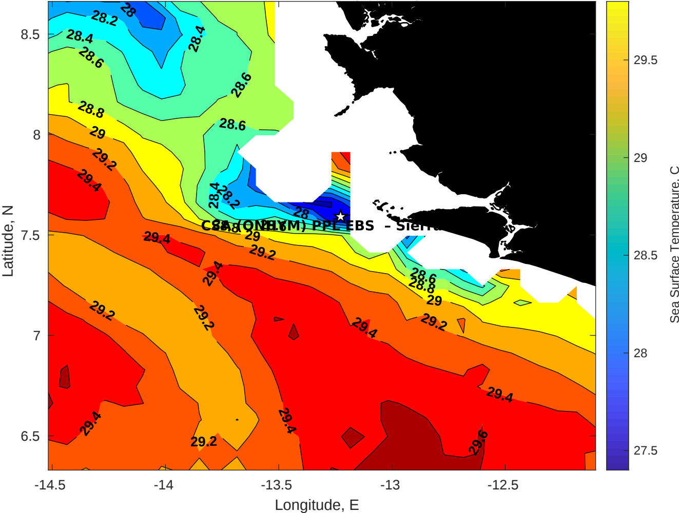
SST for CSA (ONHYM) PPL EBS - Sierra Leone at 19-May-2025 00:00:00
