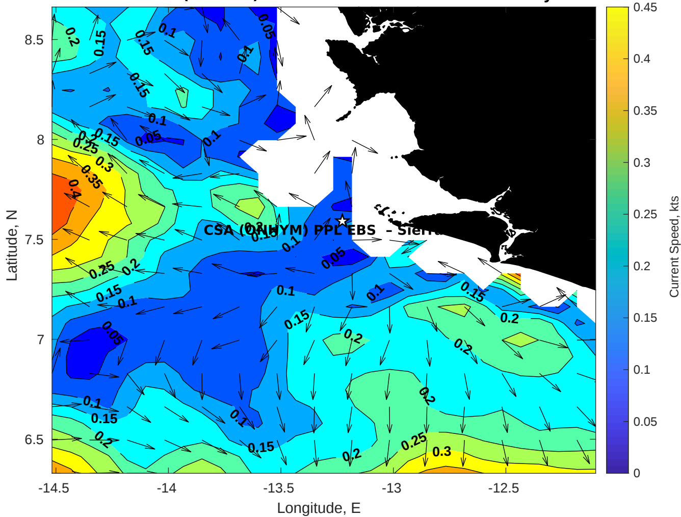
Surface Currents for CSA (ONHYM) PPL EBS - Sierra Leone at 19-May-2025 00:00:00
