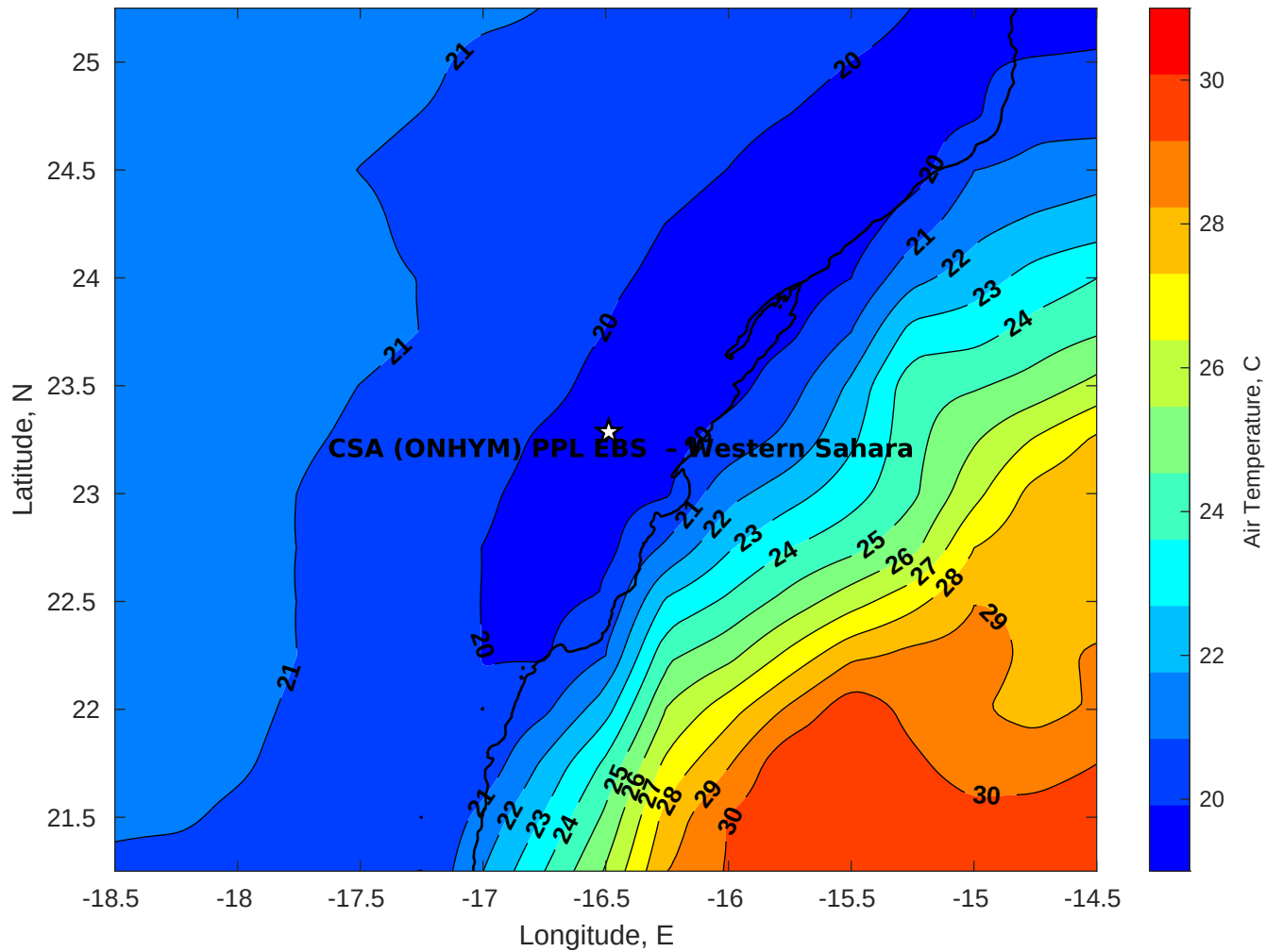
Air Temperature (C) for CSA (ONHYM) PPL EBS - Western Sahara at 20-May-2025
