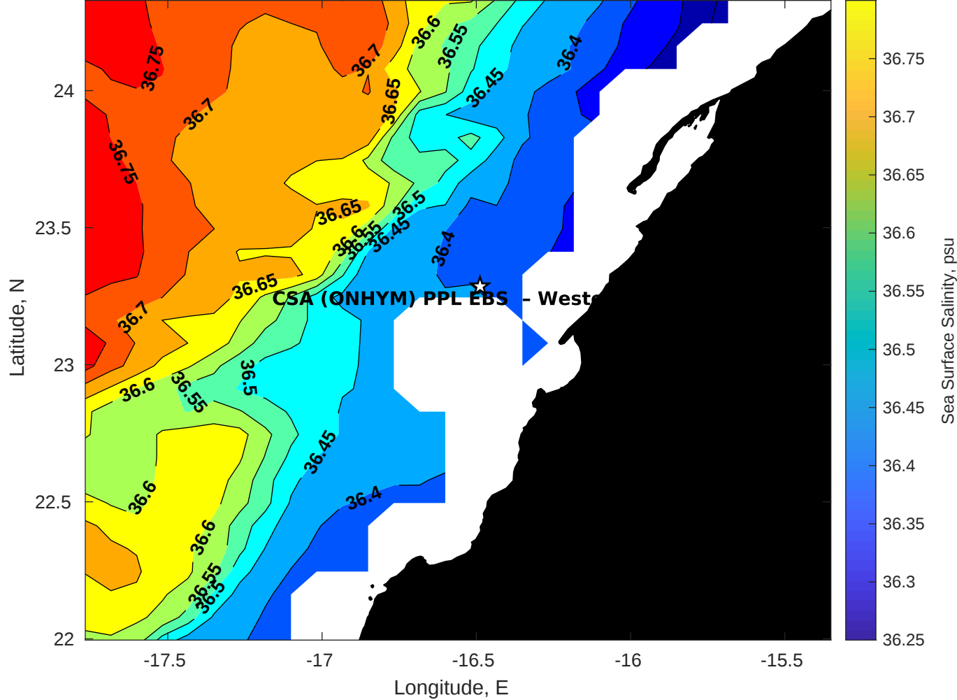
Surface Salinity for CSA (ONHYM) PPL EBS - Western Sahara at 19-May-2025 00:00:00
