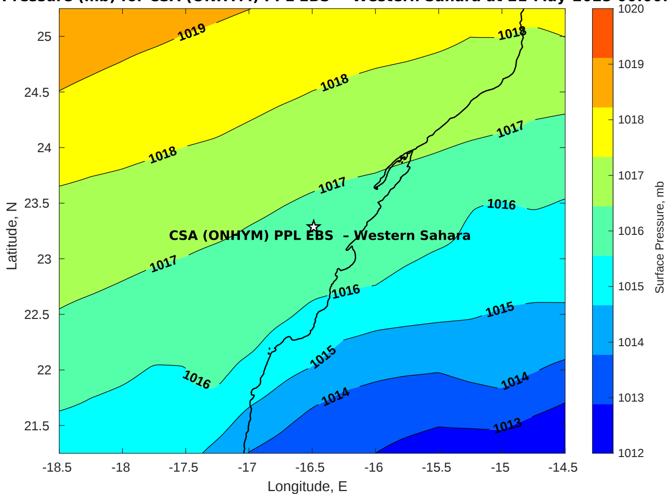
Surface Pressure (mb) for CSA (ONHYM) PPL EBS - Western Sahara at 21-May-2025 00:00:00
