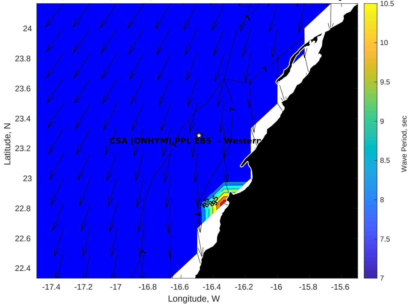
Wave Period (sec) for CSA (ONHYM) PPL EBS - Western Sahara at 20-May-2025 09:00:00
