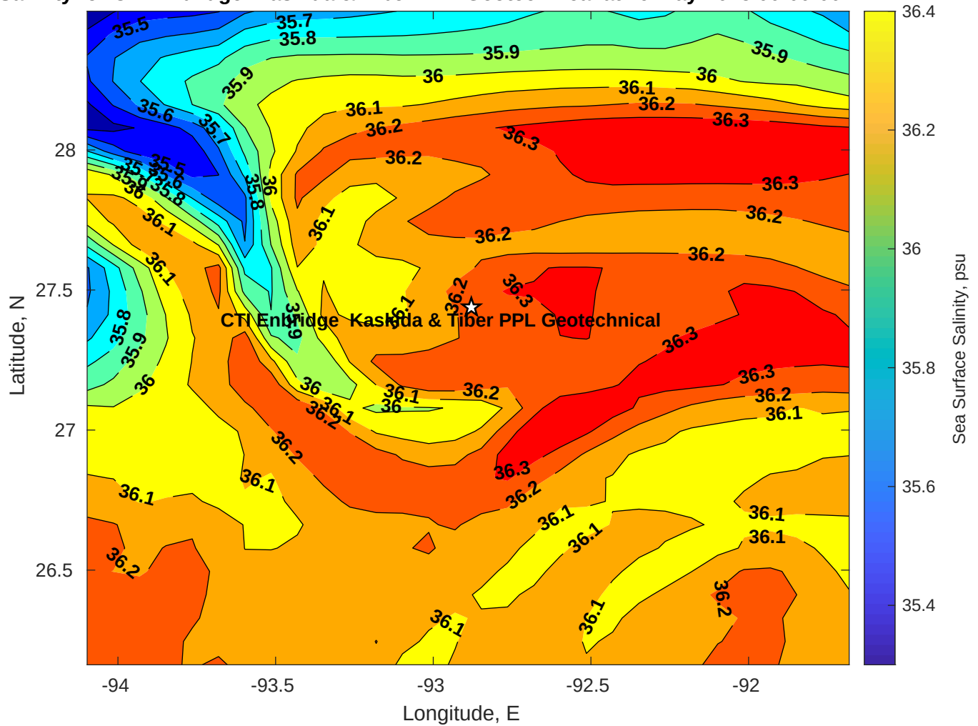
Surface Salinity for CTI Enbridge Kaskida & Tiber PPL Geotechnical at 19-May-2025 00:00:00
