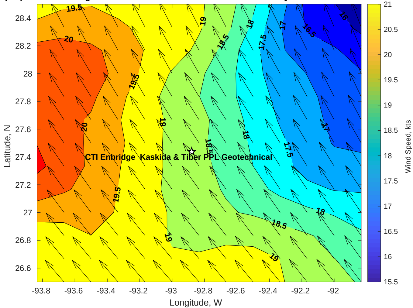
Winds (kts) for CTI Enbridge Kaskida & Tiber PPL Geotechnical at 20-May-2025 09:00:00
