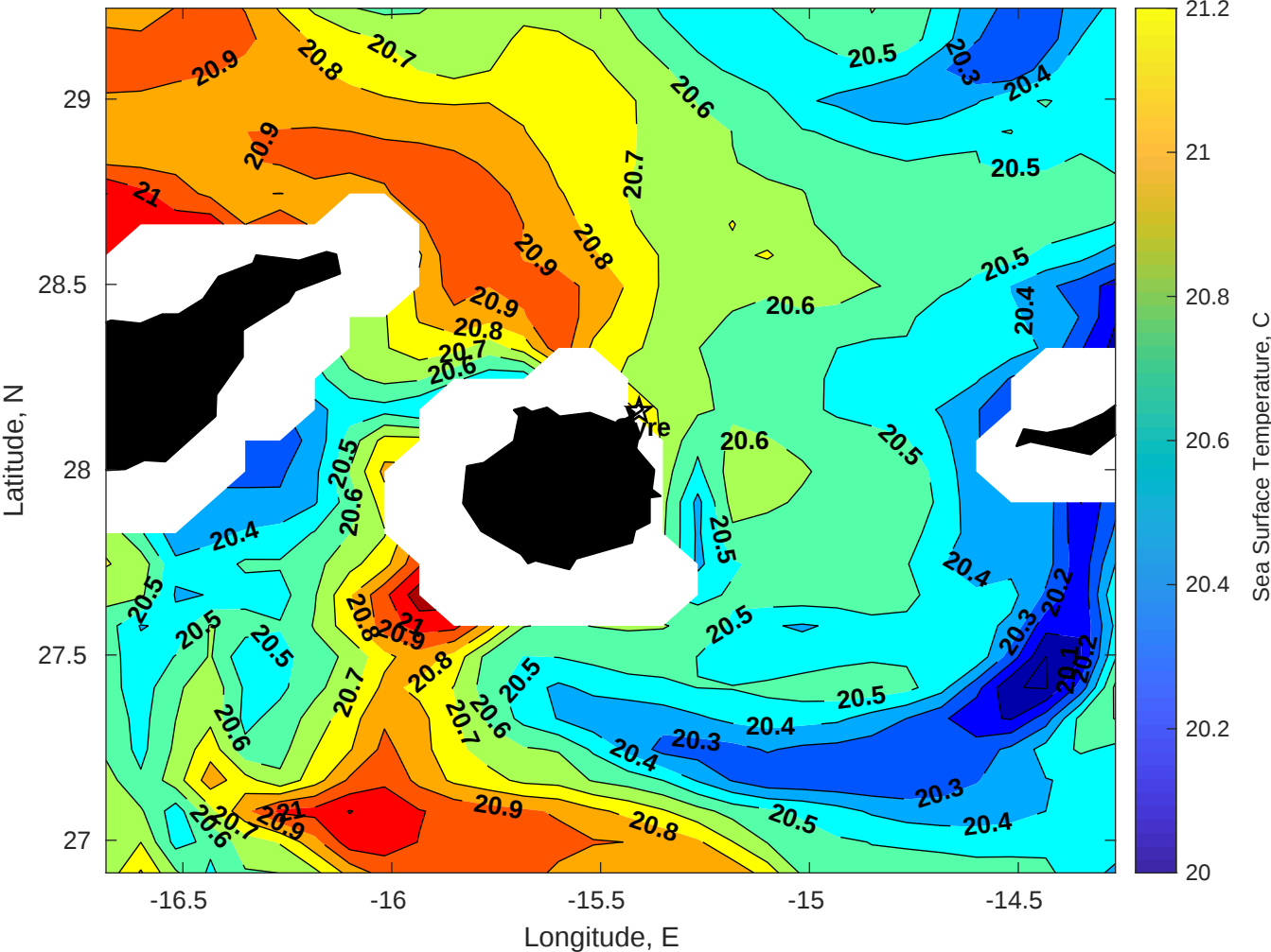
SST for Gyre at 19-May-2025 00:00:00
