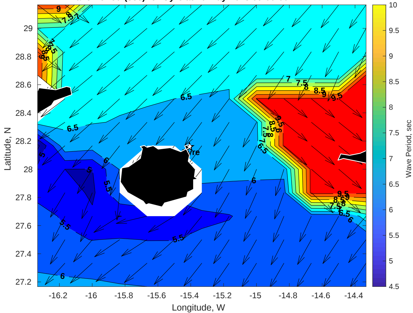
Wave Period (sec) for Gyre at 20-May-2025 09:00:00
