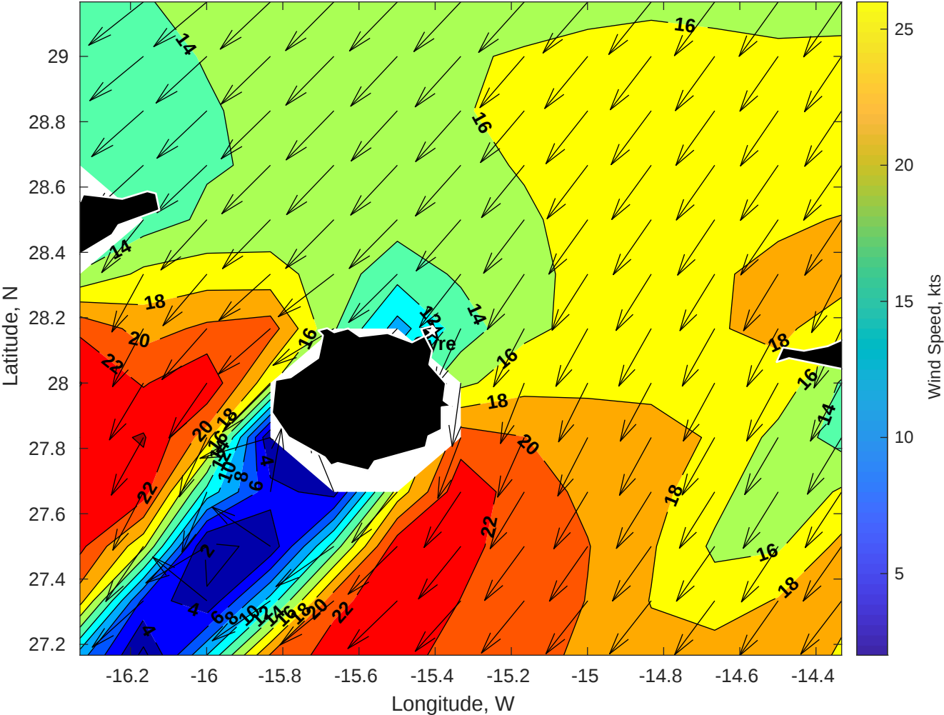
Winds (kts) for Gyre at 20-May-2025 09:00:00
