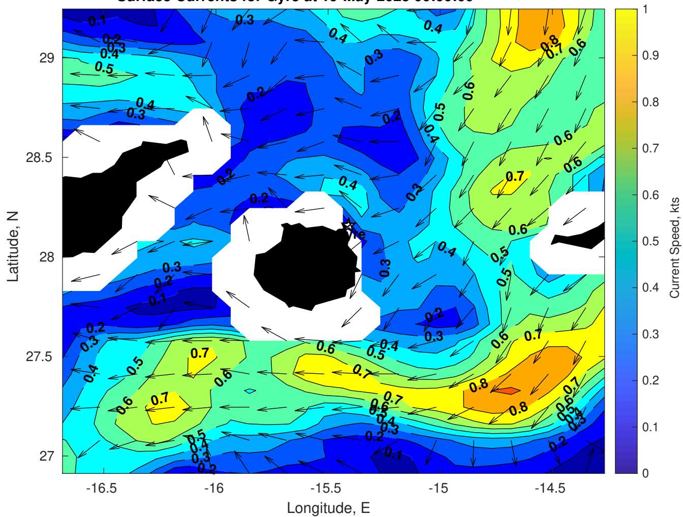
Surface Currents for Gyre at 19-May-2025 00:00:00
