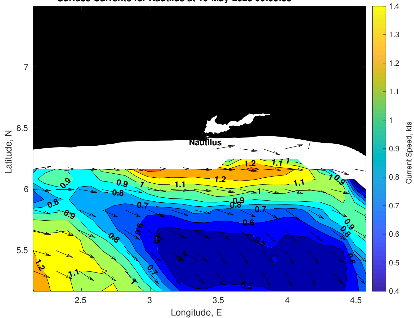
Surface Currents for Nautilus at 19-May-2025 00:00:00
