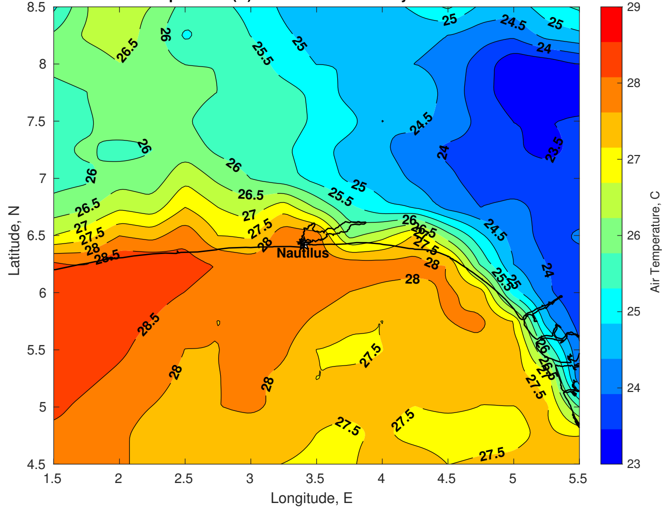
Air Temperature (C) for Nautilus at 20-May-2025
