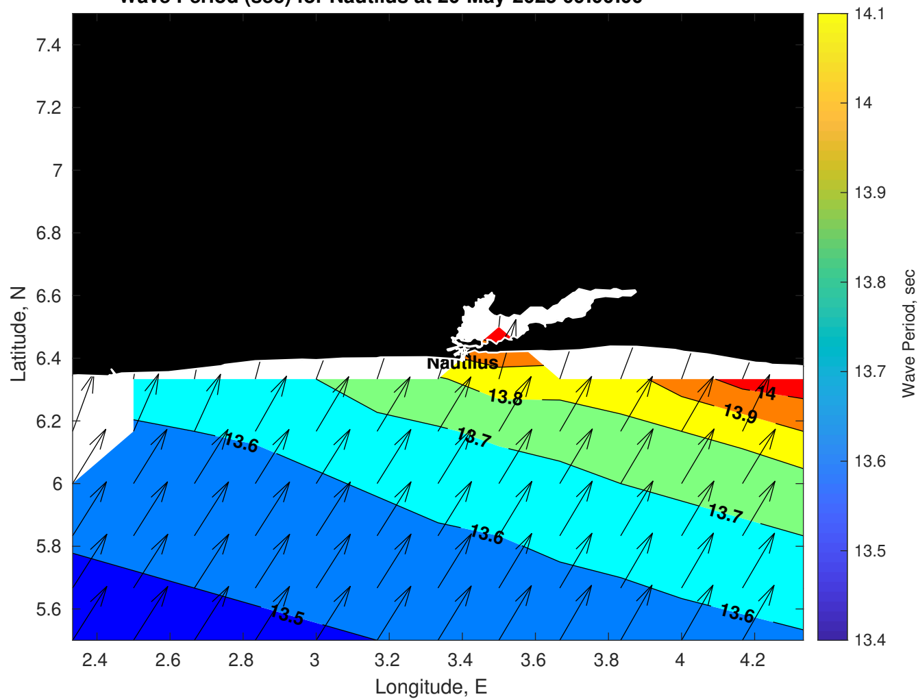
Wave Period (sec) for Nautilus at 20-May-2025 09:00:00
