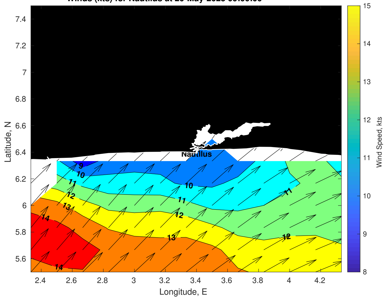
Winds (kts) for Nautilus at 20-May-2025 09:00:00
