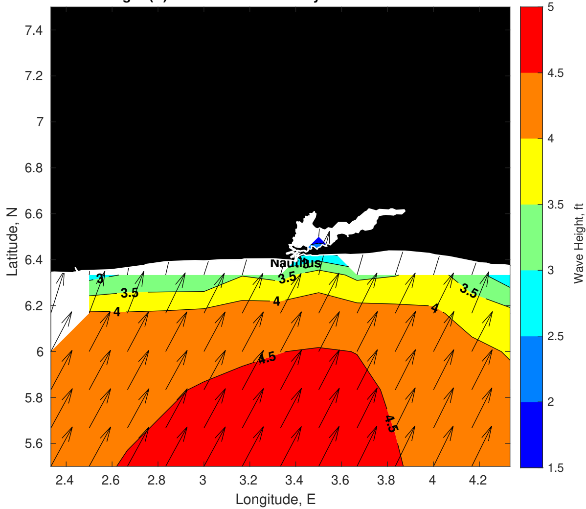
Wave Height (ft) for Nautilus at 20-May-2025 09:00:00
