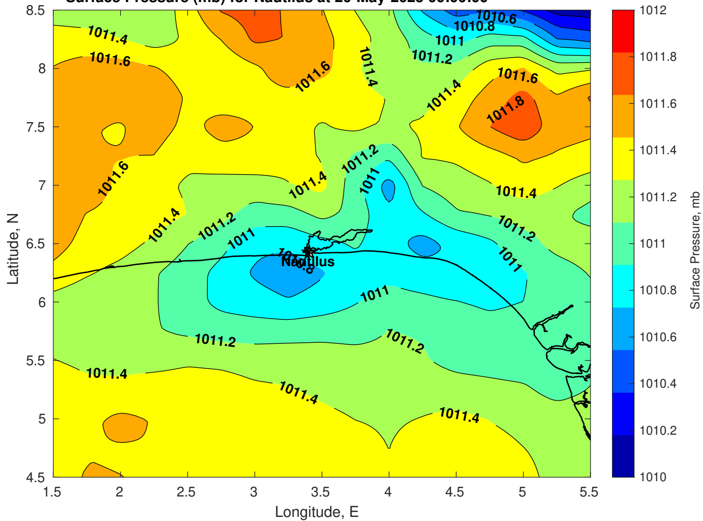
Surface Pressure (mb) for Nautilus at 20-May-2025 00:00:00
