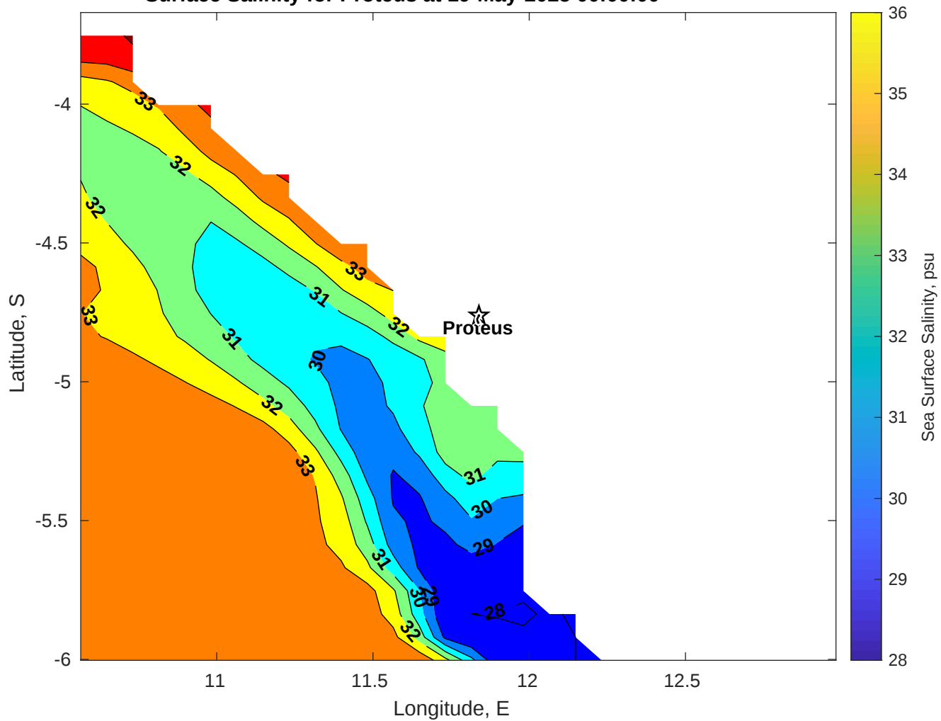
Surface Salinity for Proteus at 19-May-2025 00:00:00
