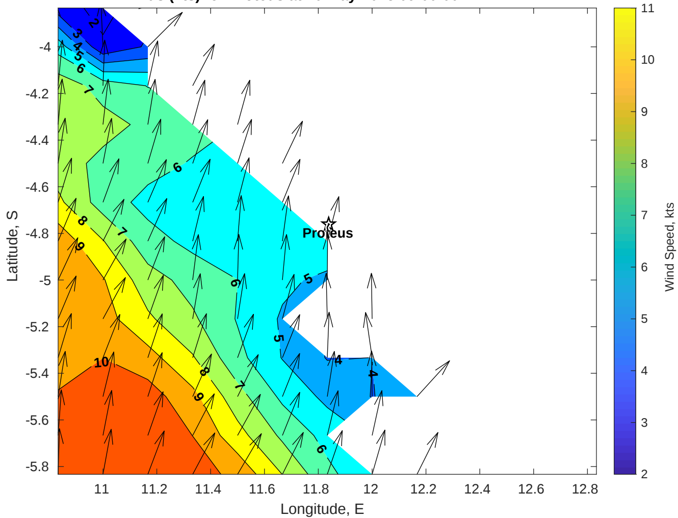
Winds (kts) for Proteus at 20-May-2025 09:00:00
