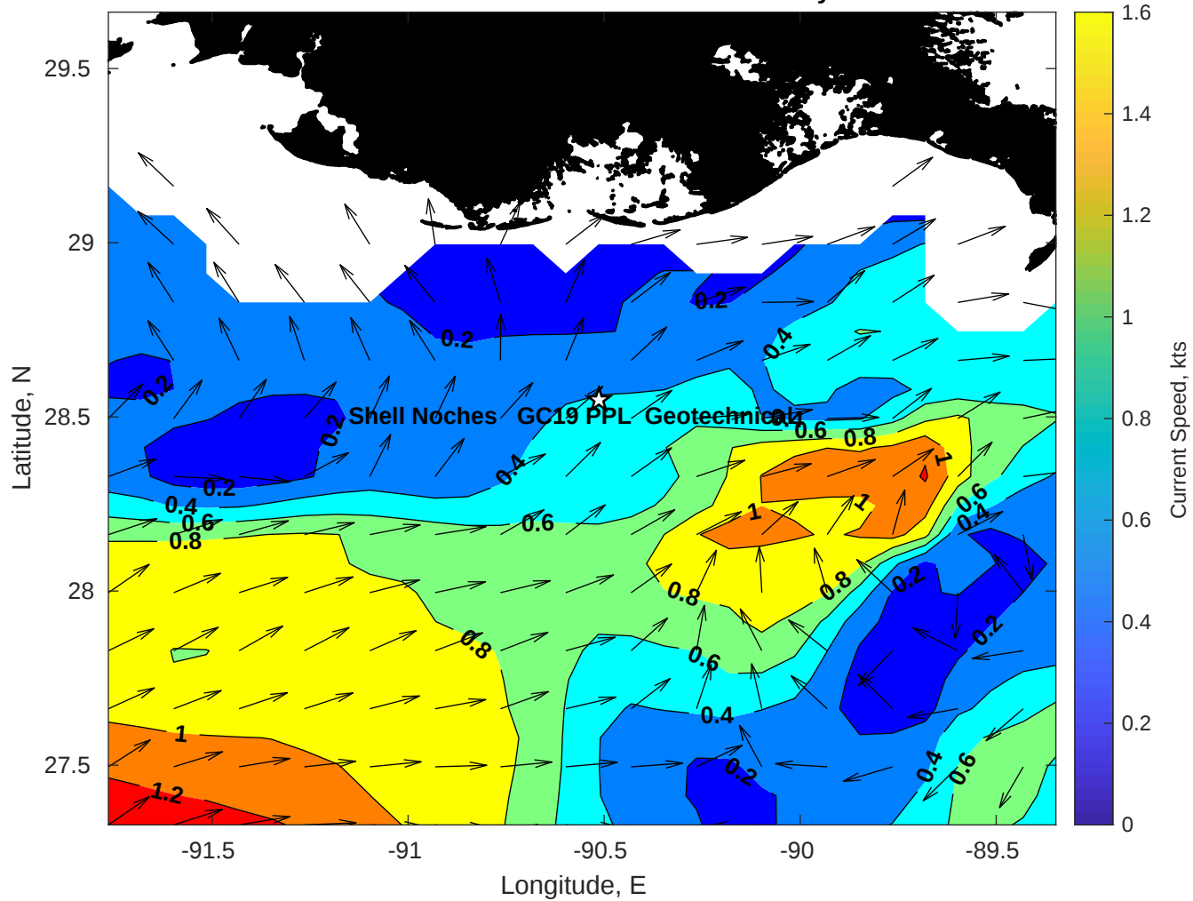
Surface Currents for Shell Noches GC19 PPL Geotechnical at 19-May-2025 00:00:00
