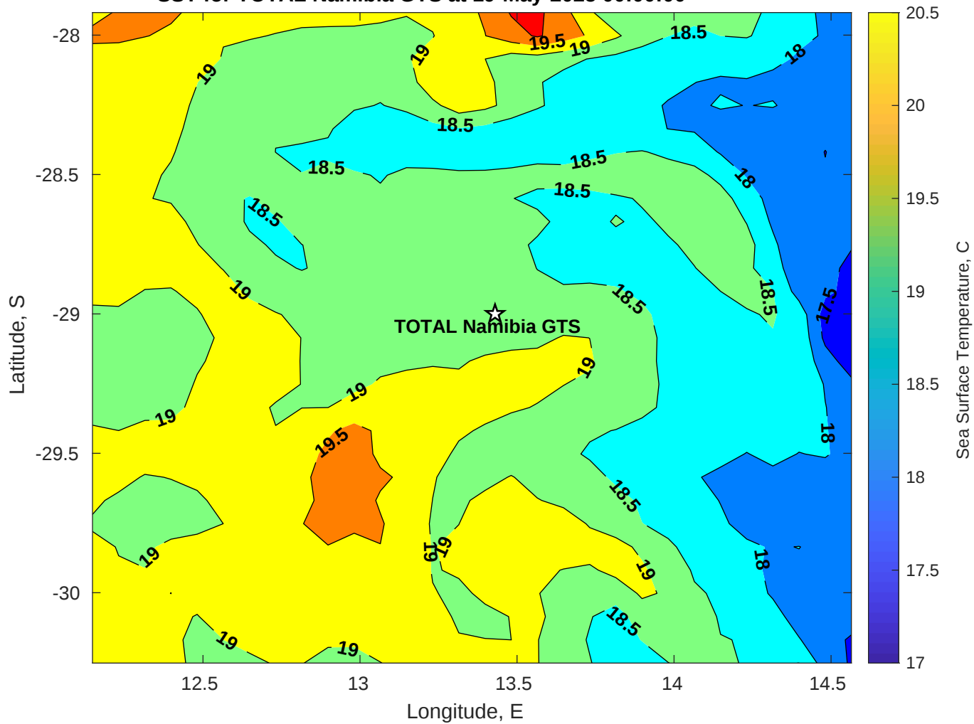
SST for TOTAL Namibia GTS at 19-May-2025 00:00:00
