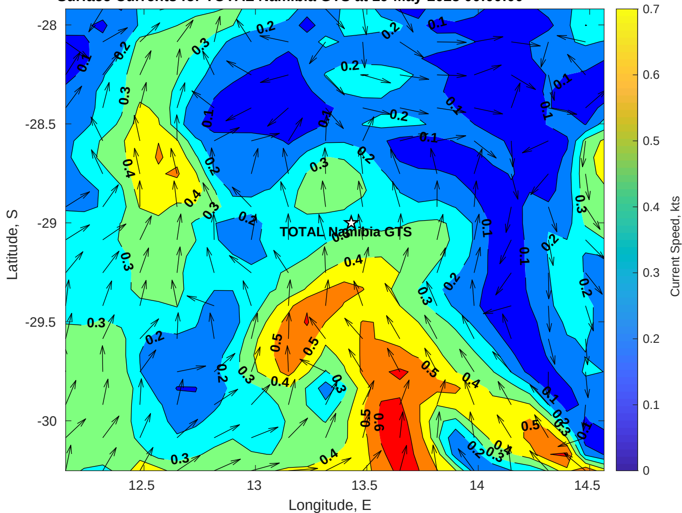
Surface Currents for TOTAL Namibia GTS at 19-May-2025 00:00:00
