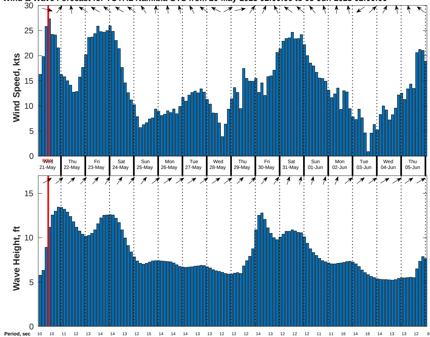
Wind & Wave Forecast for TOTAL Namibia GTS from 20-May-2025 02:00:00 to 05-Jun-2025 02:00:00
