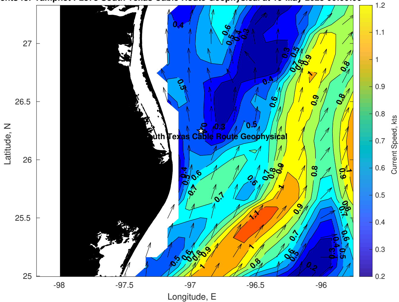
Surface Currents for Tampnet P2378 South Texas Cable Route Geophysical at 19-May-2025 00:00:00
