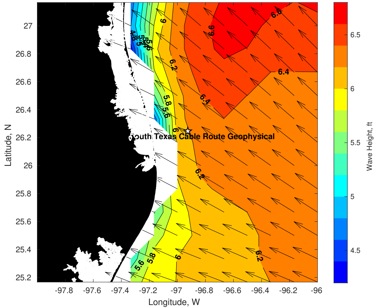
Wave Height (ft) for Tampnet P2378 South Texas Cable Route Geophysical at 20-May-2025 09:00:00
