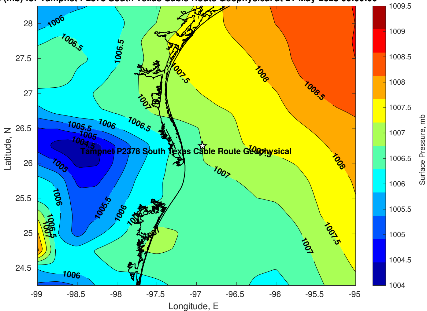
Pressure (mb) for Tampnet P2378 South Texas Cable Route Geophysical at 21-May-2025 00:00:00
