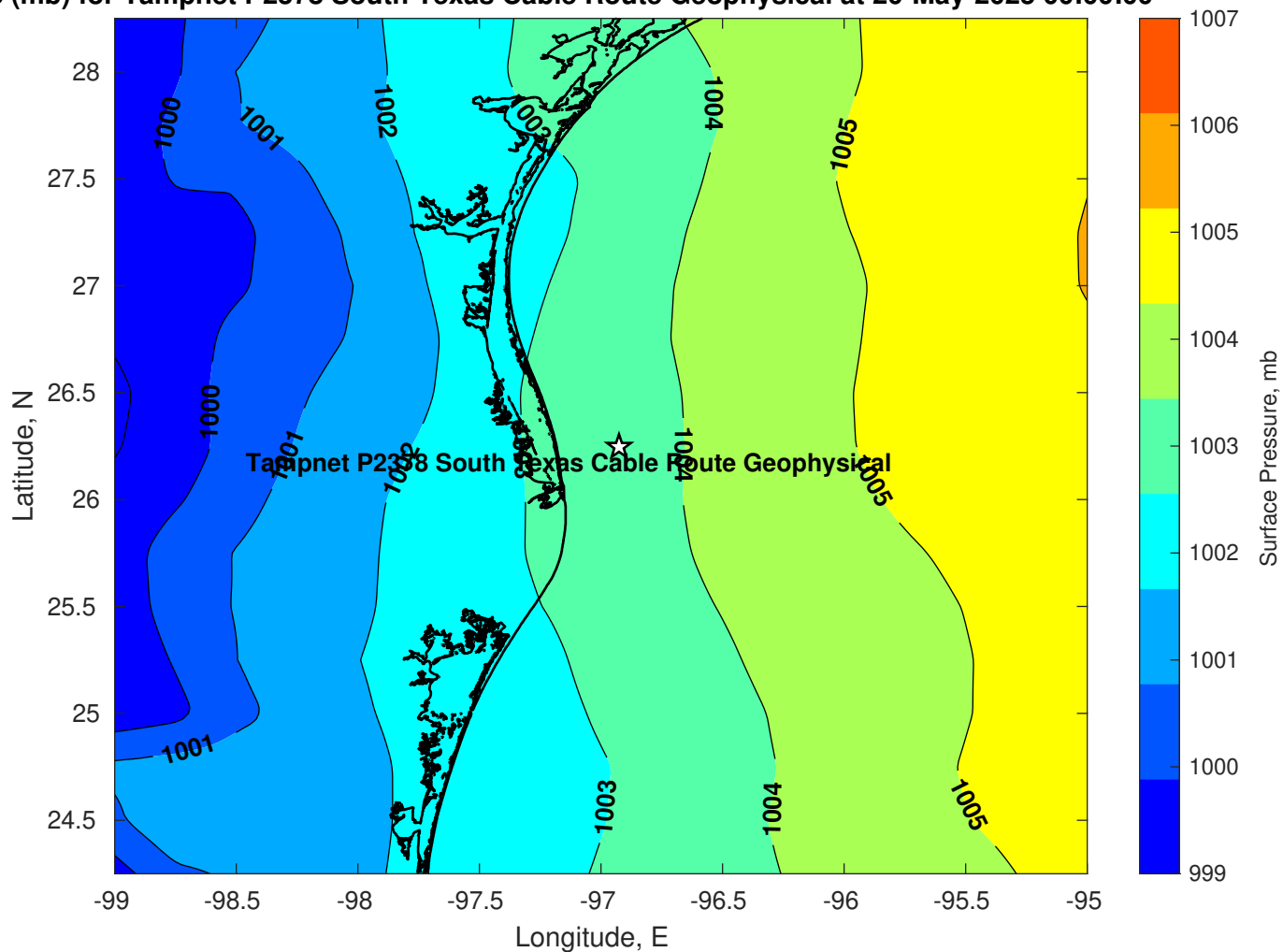
Pressure (mb) for Tampnet P2378 South Texas Cable Route Geophysical at 20-May-2025 00:00:00
