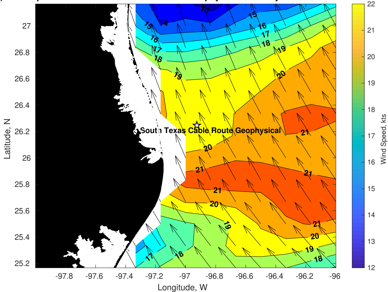
Winds (kts) for Tampnet P2378 South Texas Cable Route Geophysical at 20-May-2025 09:00:00
