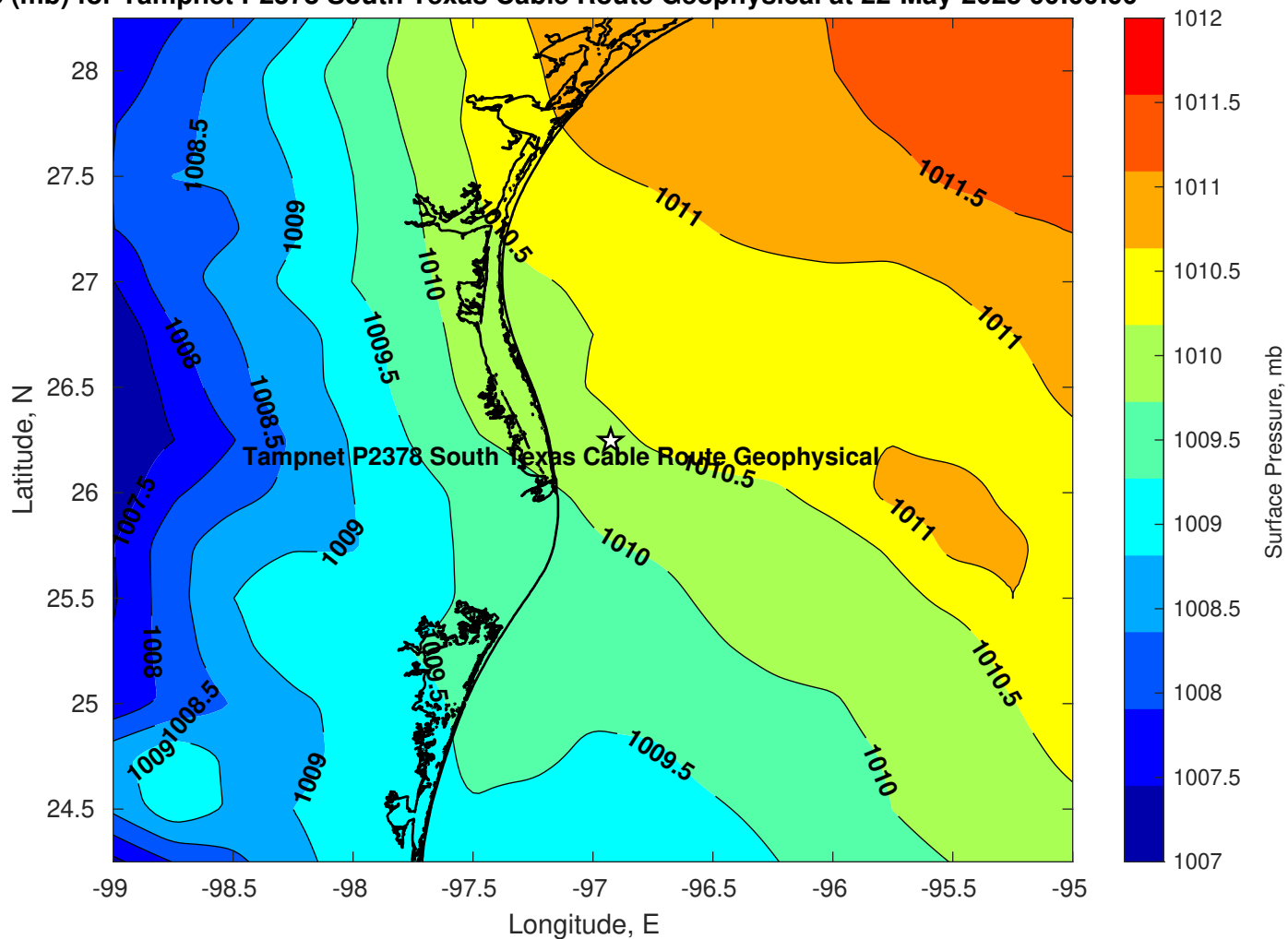
Pressure (mb) for Tampnet P2378 South Texas Cable Route Geophysical at 22-May-2025 00:00:00
