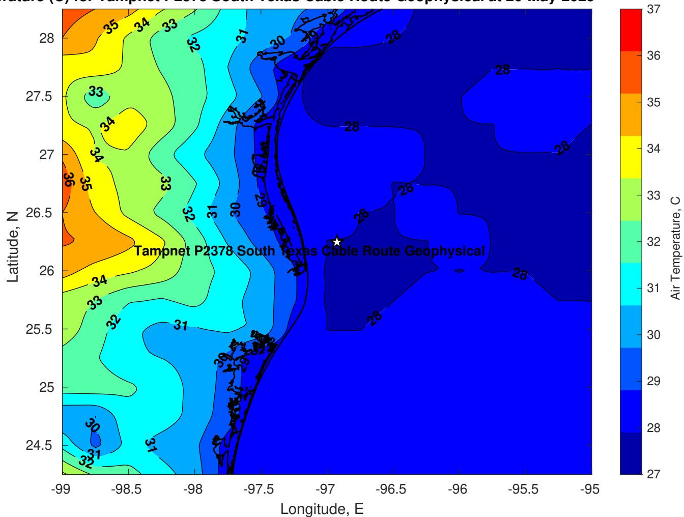
Air Temperature (C) for Tampnet P2378 South Texas Cable Route Geophysical at 20-May-2025
