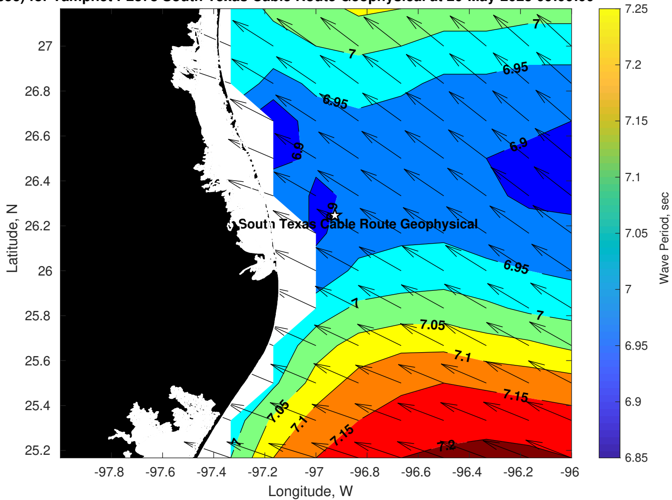
Period (sec) for Tampnet P2378 South Texas Cable Route Geophysical at 20-May-2025 09:00:00
