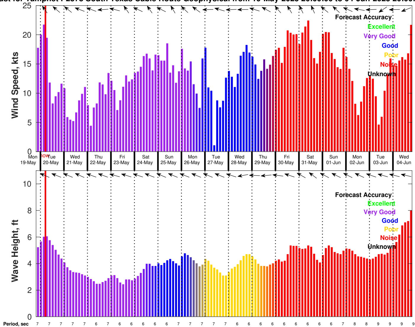
Wind & Wave Forecast for Tampnet P2378 South Texas Cable Route Geophysical from 19-May-2025 20:00:00 to 04-Jun-2025 20:00:00
