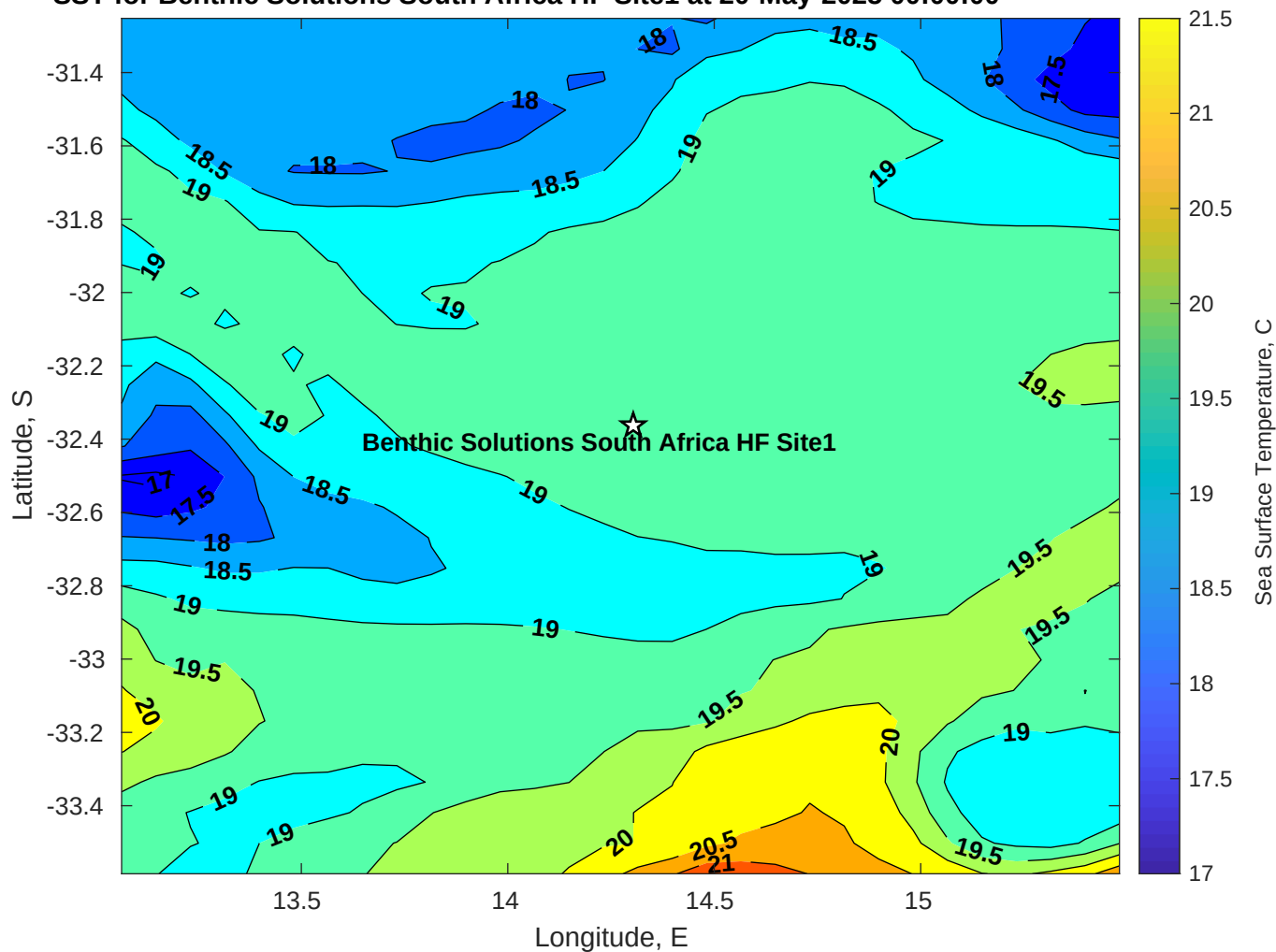
SST for Benthic Solutions South Africa HF Site1 at 20-May-2025 00:00:00
