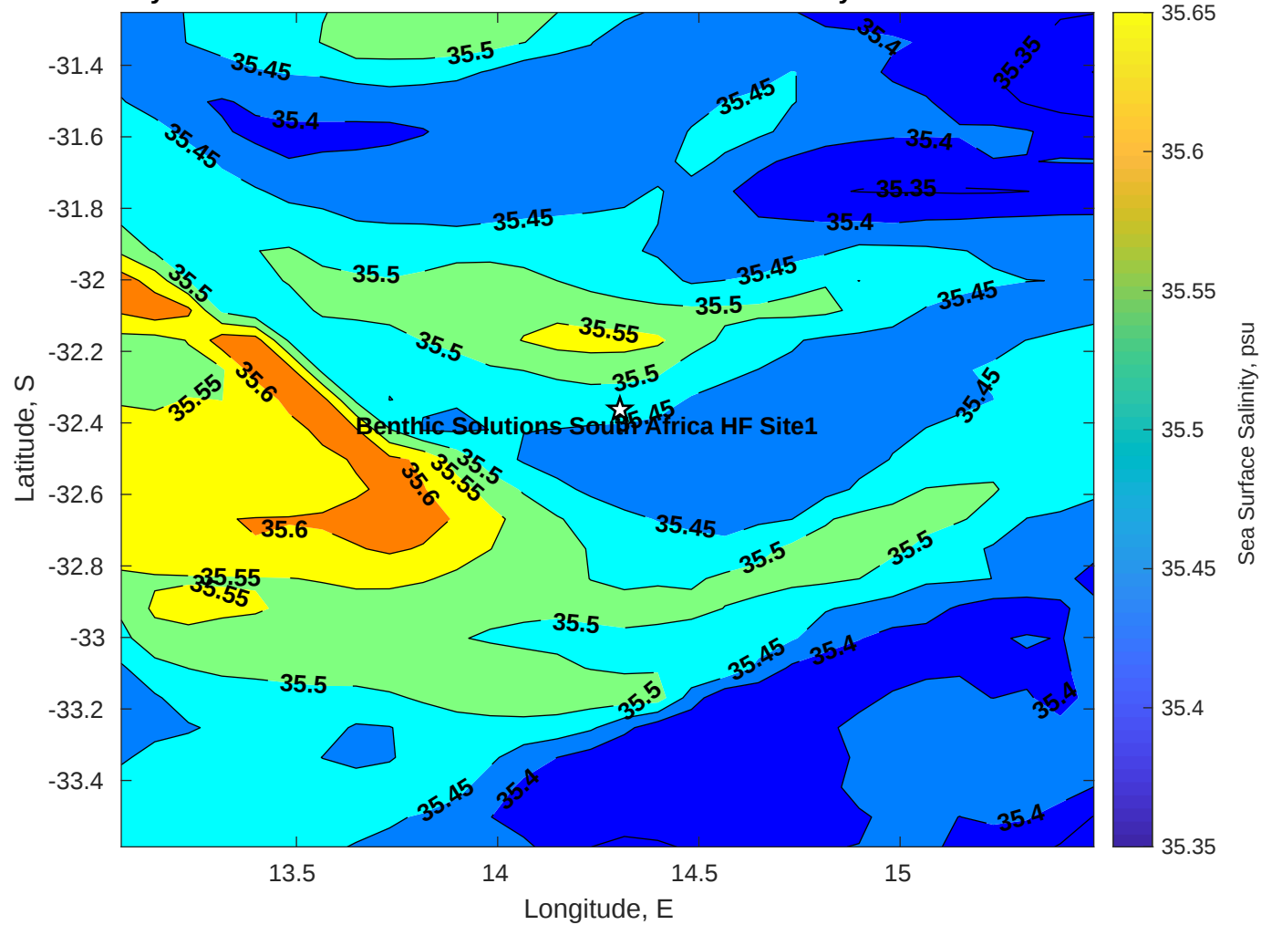
Surface Salinity for Benthic Solutions South Africa HF Site1 at 20-May-2025 00:00:00
