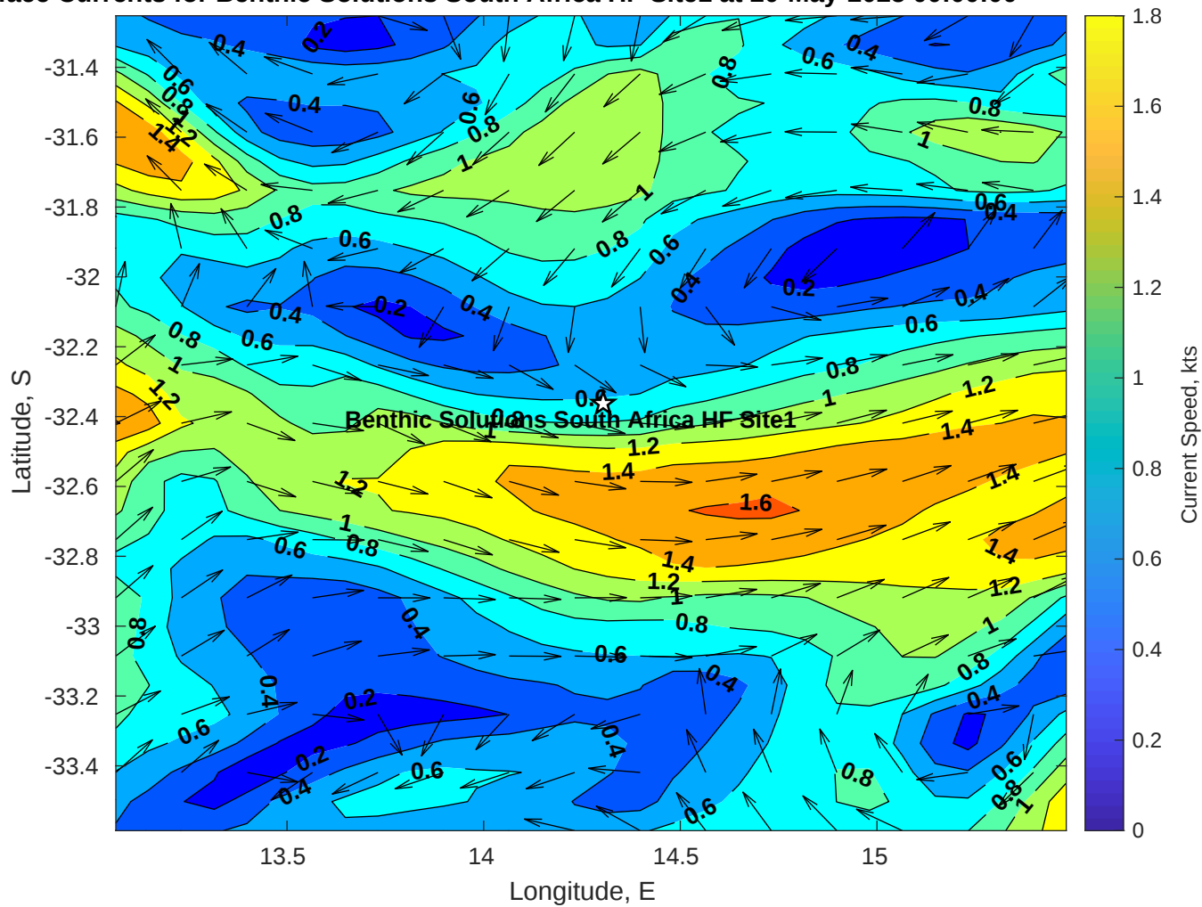
Surface Currents for Benthic Solutions South Africa HF Site1 at 20-May-2025 00:00:00
