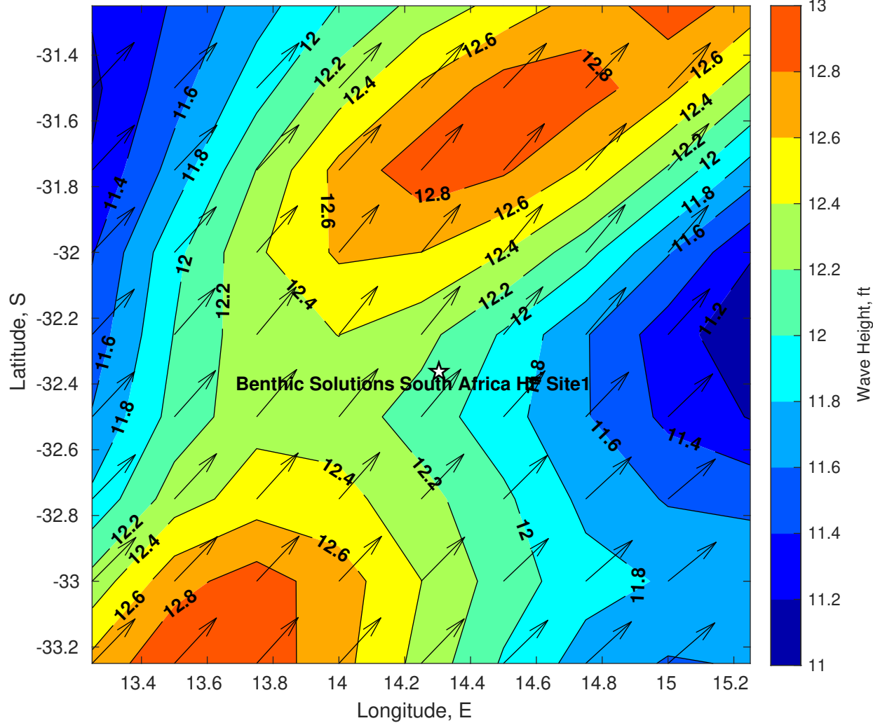
Wave Height (ft) for Benthic Solutions South Africa HF Site1 at 21-May-2025 09:00:00
