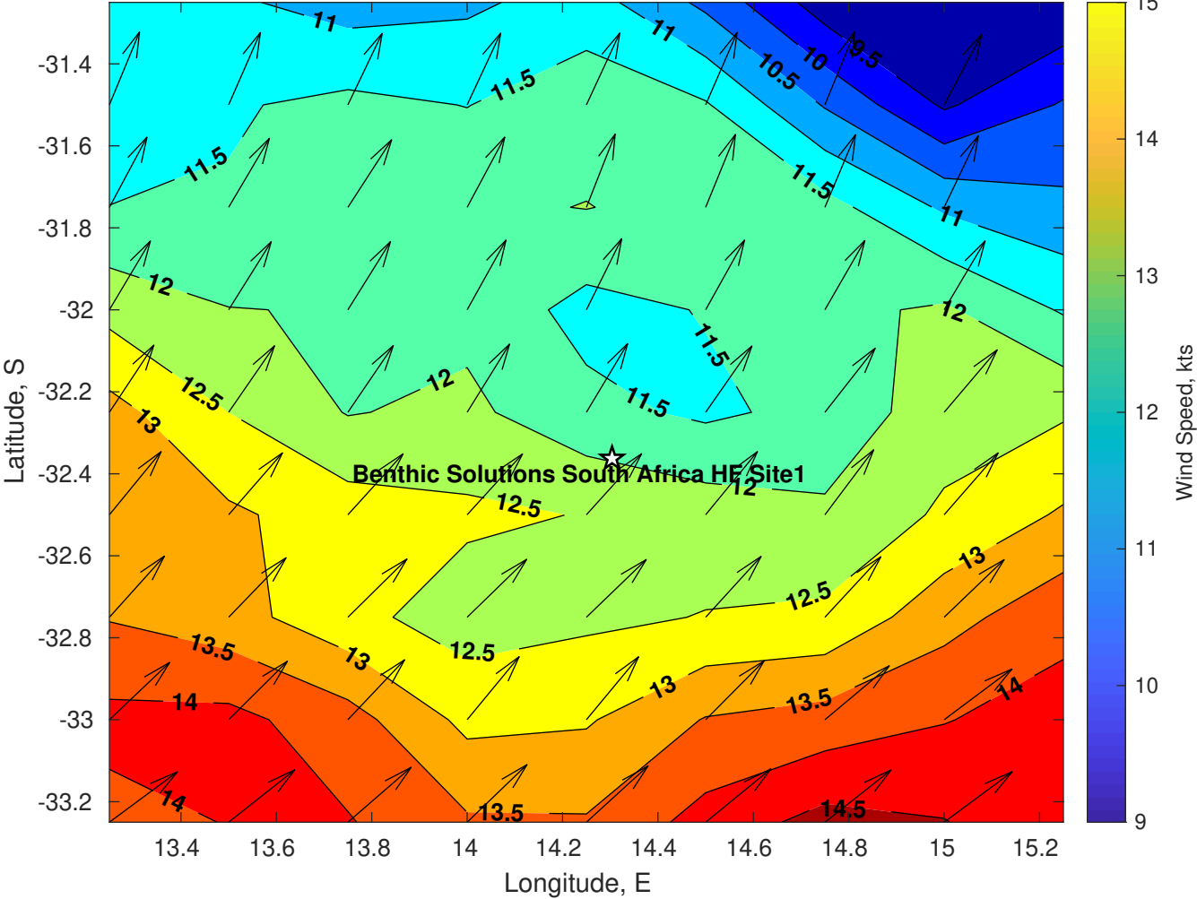
Winds (kts) for Benthic Solutions South Africa HF Site1 at 21-May-2025 09:00:00
