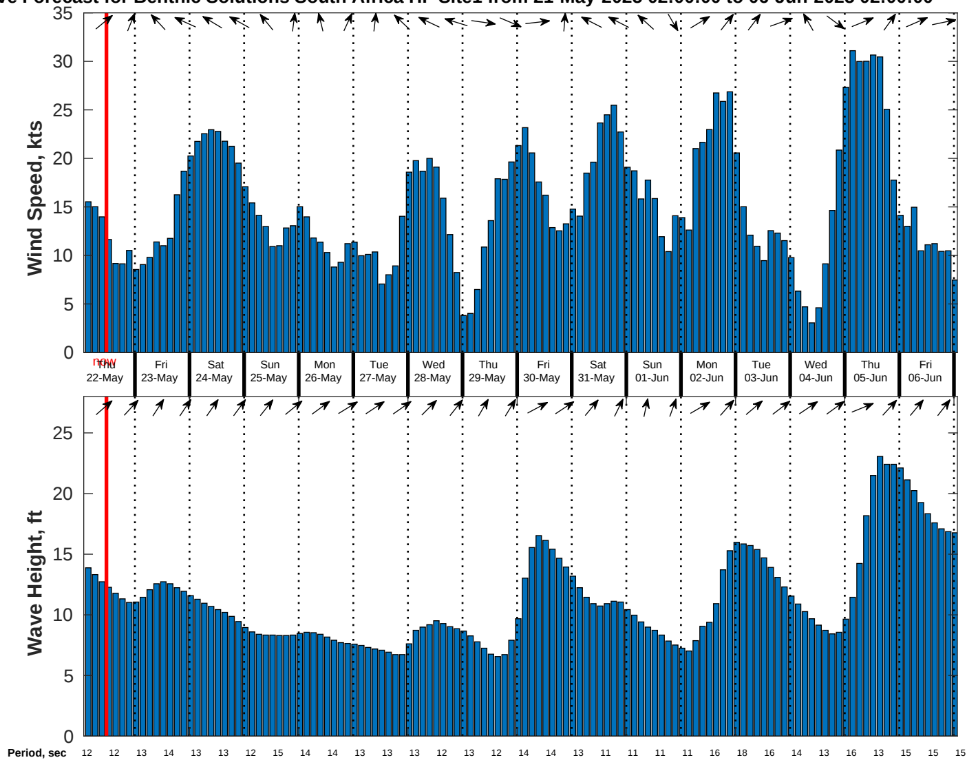
Wind & Wave Forecast for Benthic Solutions South Africa HF Site1 from 21-May-2025 02:00:00 to 06-Jun-2025 02:00:00
