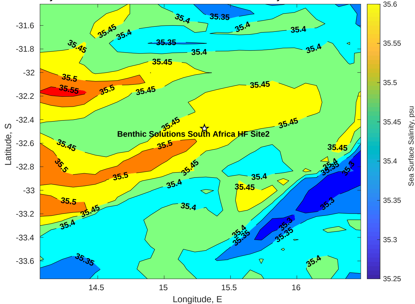
Surface Salinity for Benthic Solutions South Africa HF Site2 at 20-May-2025 00:00:00
