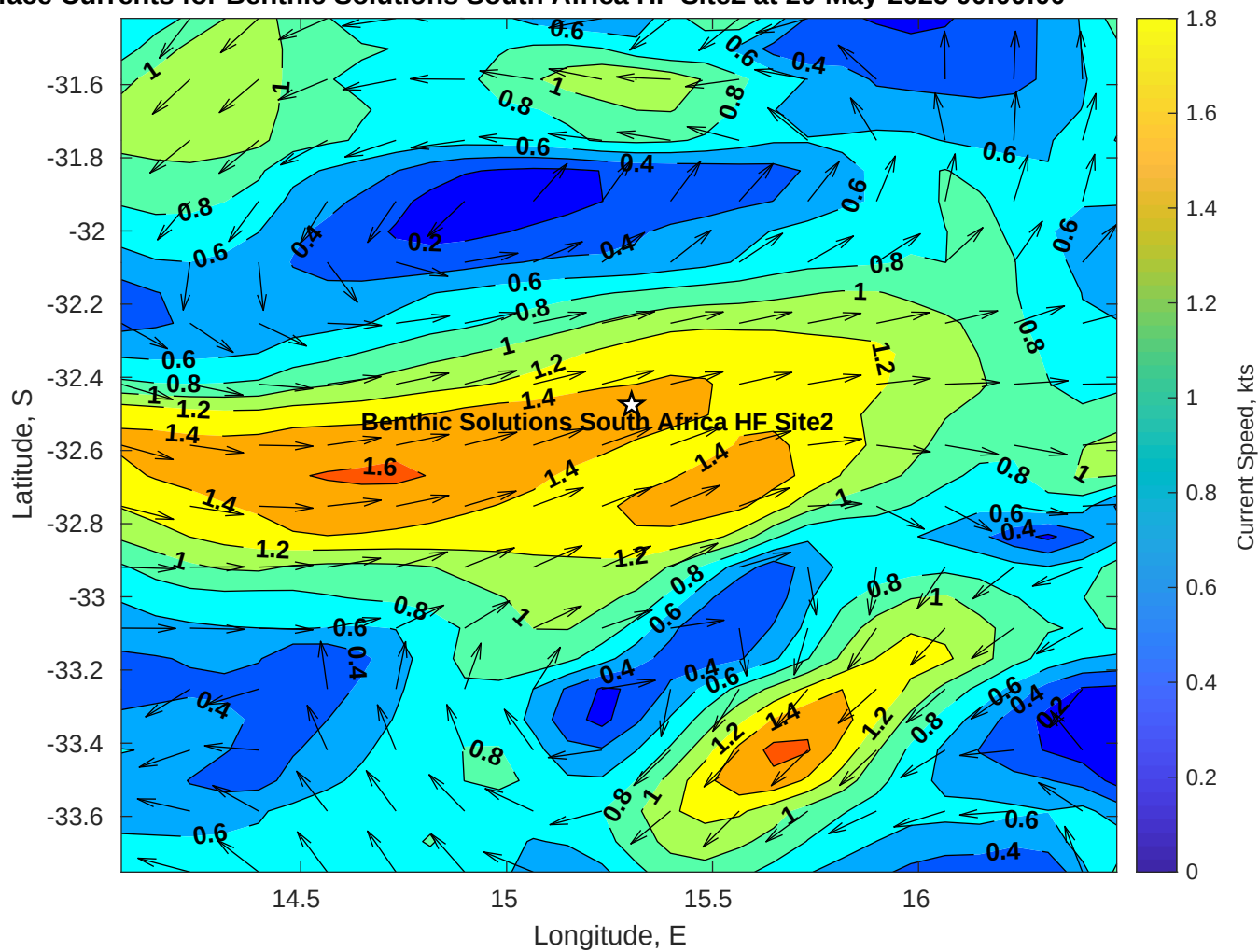
Surface Currents for Benthic Solutions South Africa HF Site2 at 20-May-2025 00:00:00
