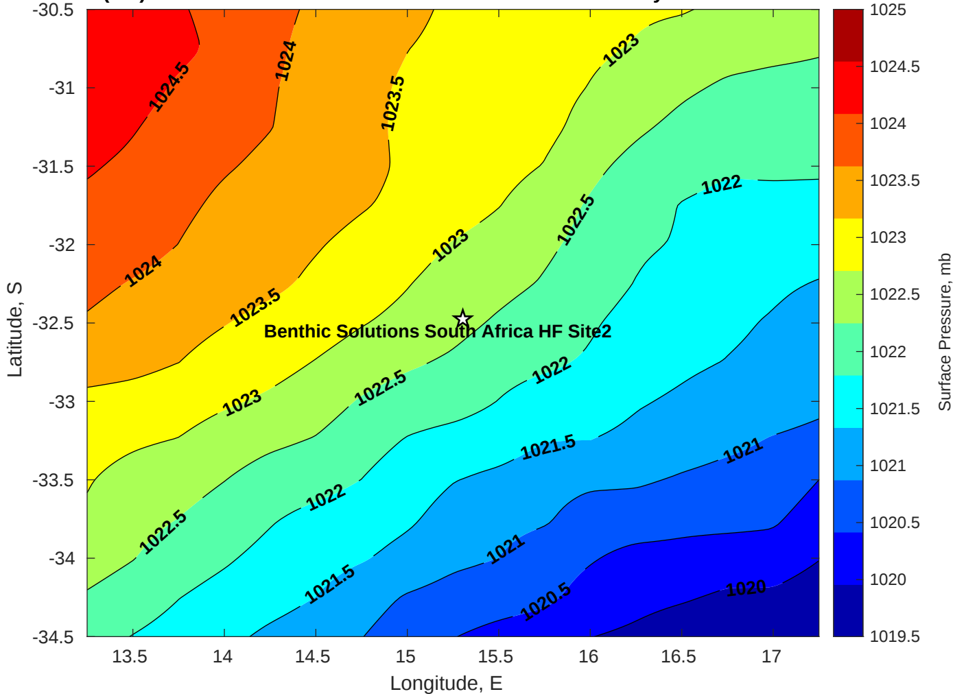
Surface Pressure (mb) for Benthic Solutions South Africa HF Site2 at 21-May-2025 00:00:00
