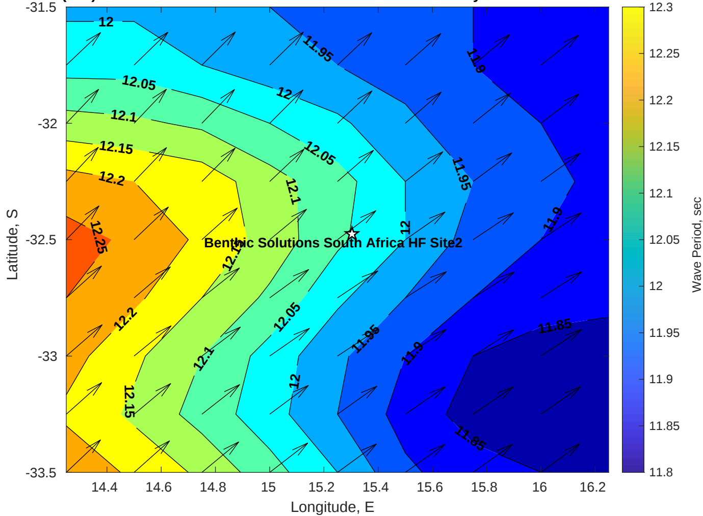
Wave Period (sec) for Benthic Solutions South Africa HF Site2 at 21-May-2025 09:00:00
