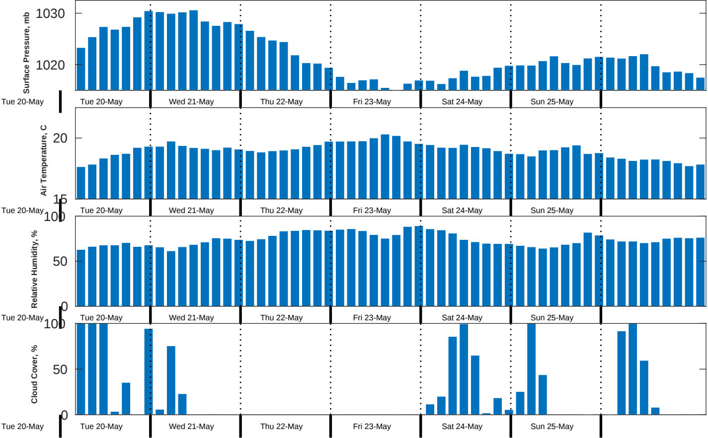
Met Forecast for Benthic Solutions South Africa HF Site2 from 21-May-2025 00:00:00 to 28-May-2025 00:00:00
