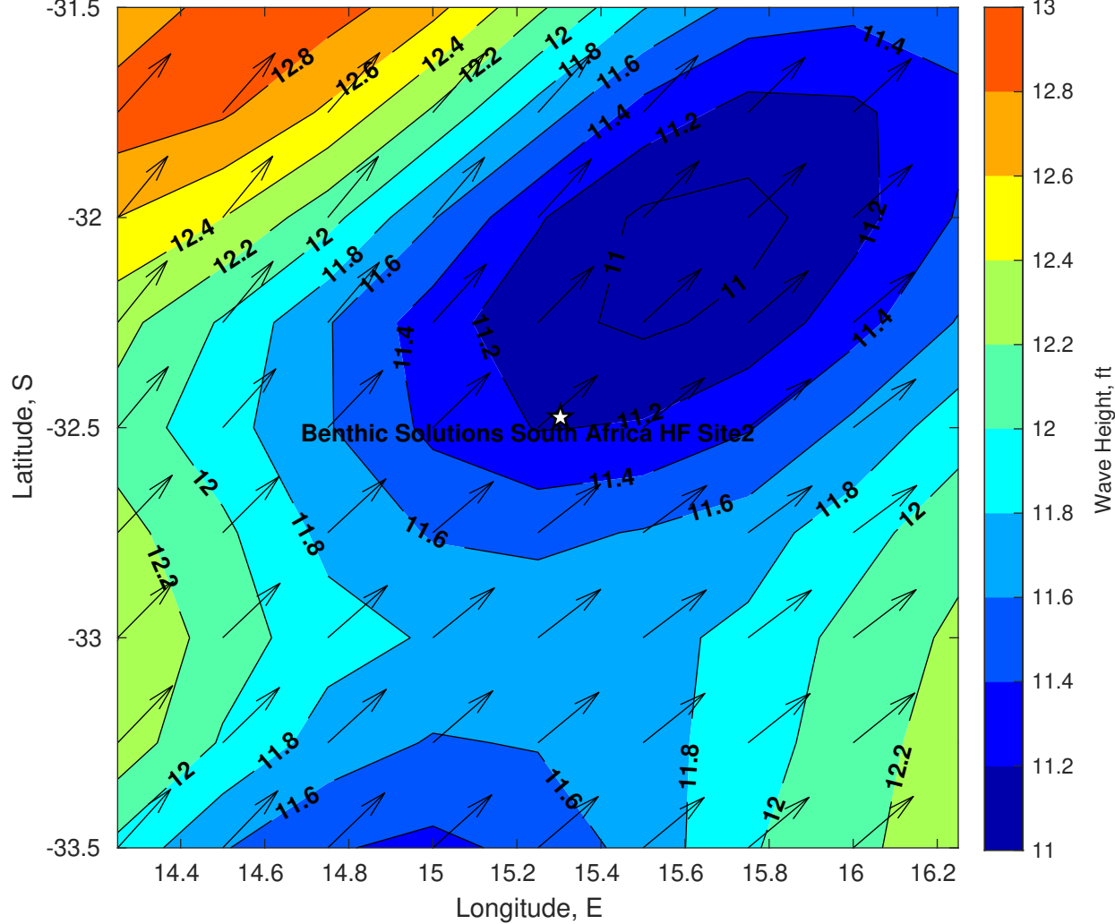
Wave Height (ft) for Benthic Solutions South Africa HF Site2 at 21-May-2025 09:00:00
