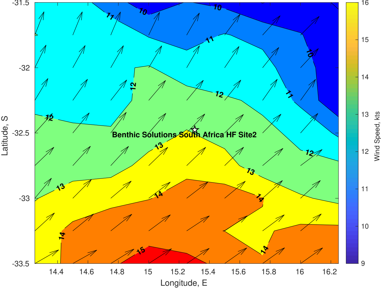
Winds (kts) for Benthic Solutions South Africa HF Site2 at 21-May-2025 09:00:00
