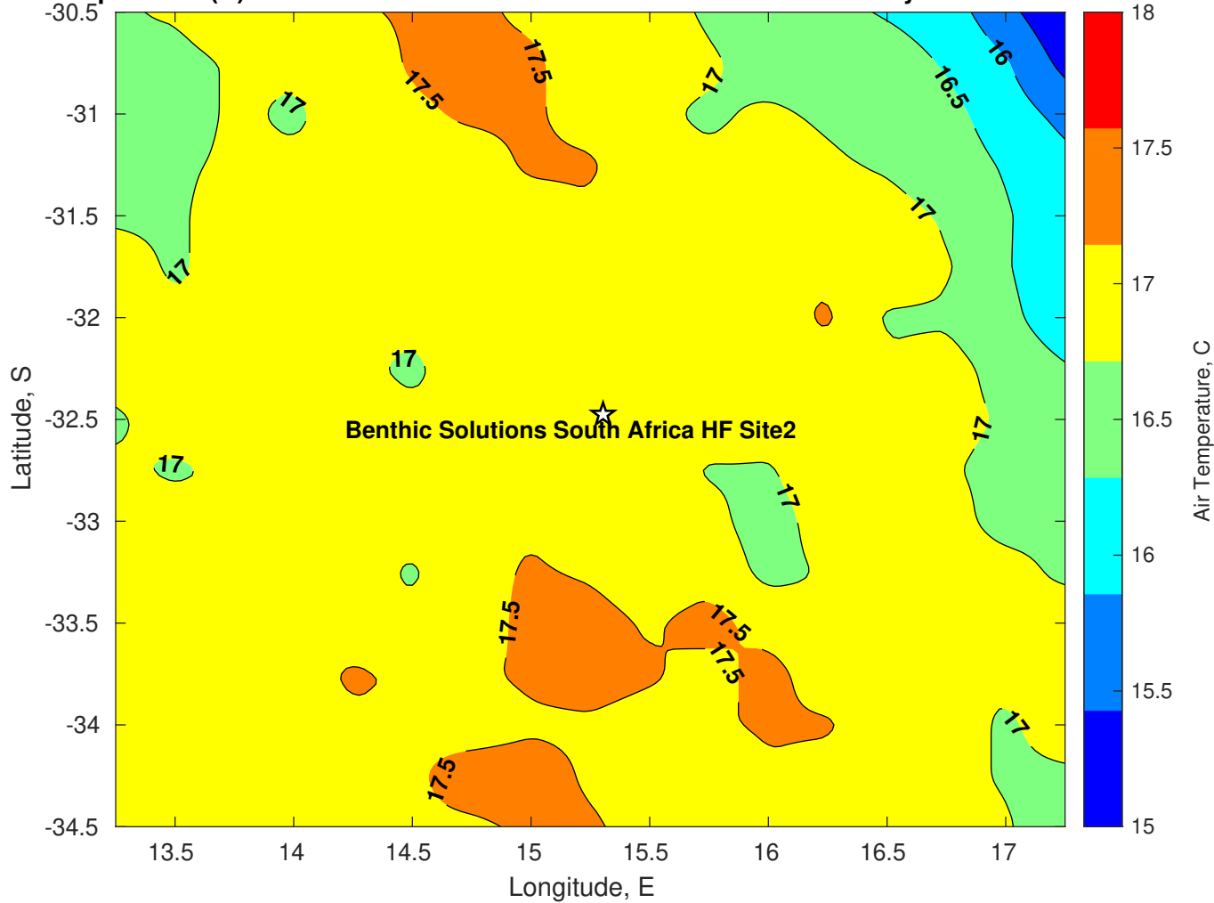
Air Temperature (C) for Benthic Solutions South Africa HF Site2 at 21-May-2025
