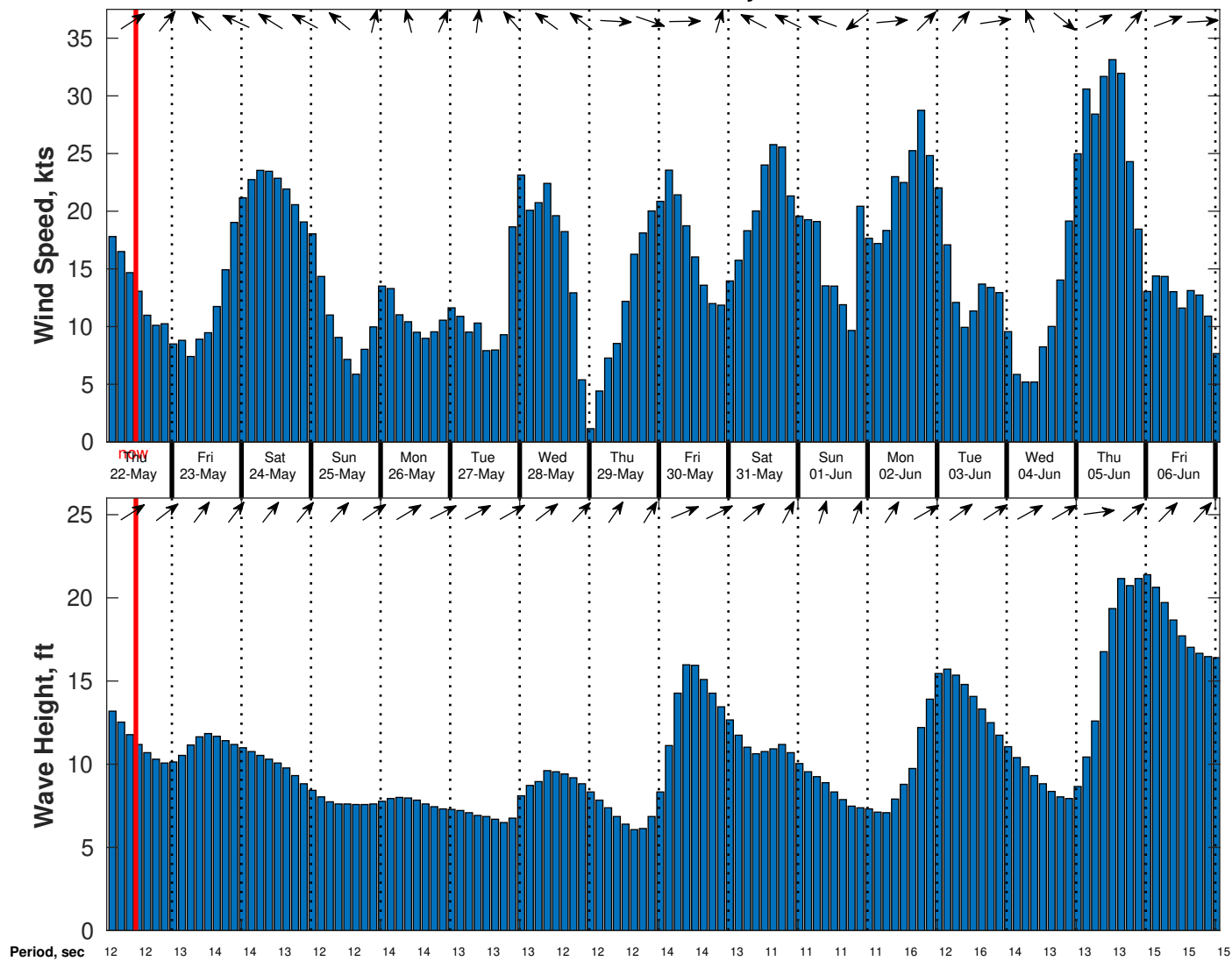
Wind & Wave Forecast for Benthic Solutions South Africa HF Site2 from 21-May-2025 02:00:00 to 06-Jun-2025 02:00:00
