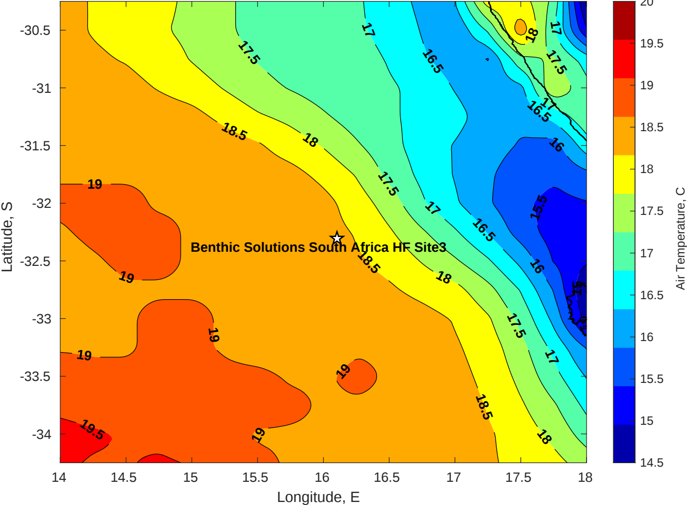
Air Temperature (C) for Benthic Solutions South Africa HF Site3 at 21-May-2025
