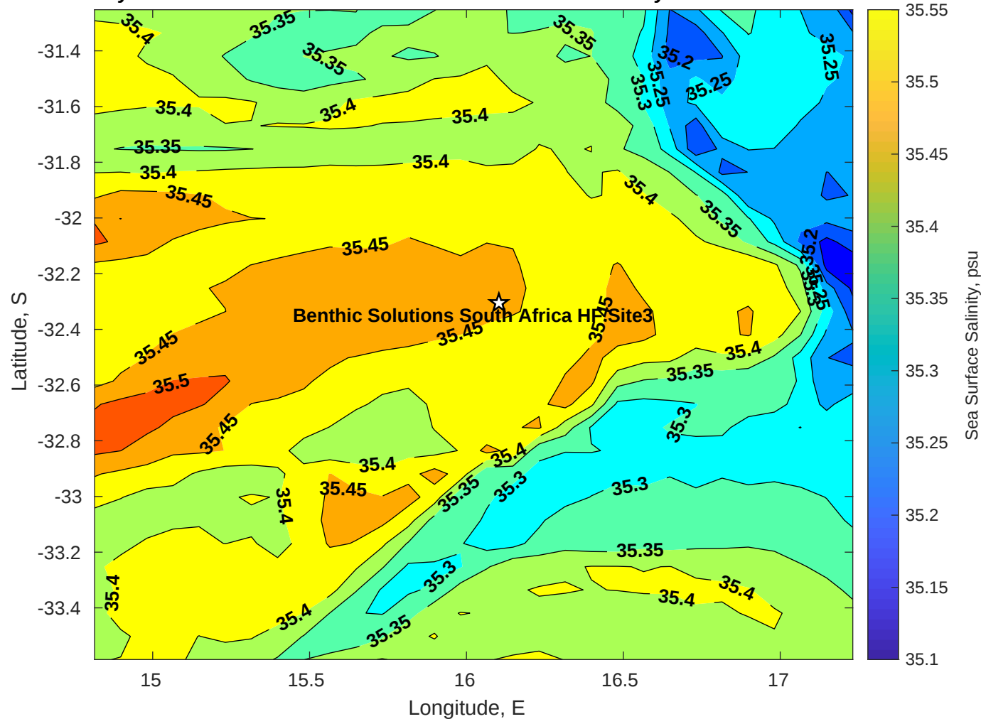
Surface Salinity for Benthic Solutions South Africa HF Site3 at 20-May-2025 00:00:00
