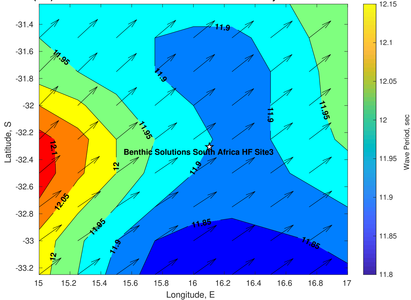
Wave Period (sec) for Benthic Solutions South Africa HF Site3 at 21-May-2025 09:00:00
