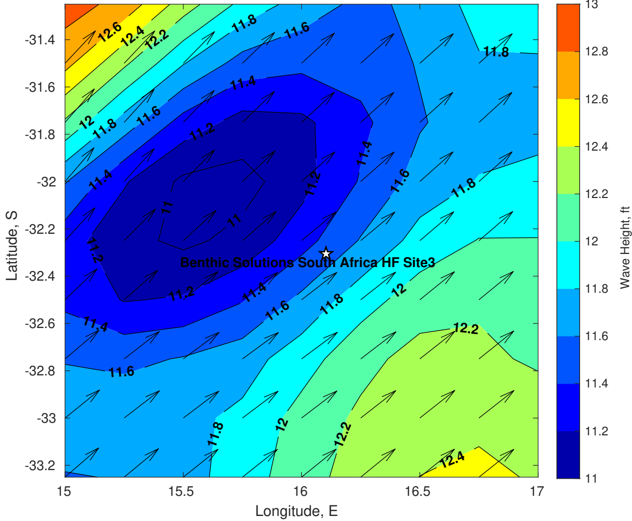
Wave Height (ft) for Benthic Solutions South Africa HF Site3 at 21-May-2025 09:00:00
