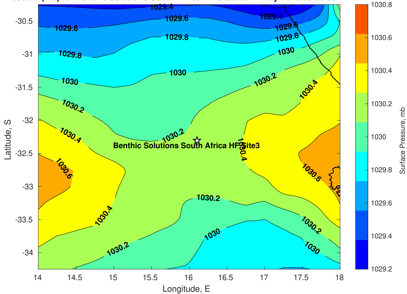
Surface Pressure (mb) for Benthic Solutions South Africa HF Site3 at 22-May-2025 00:00:00
