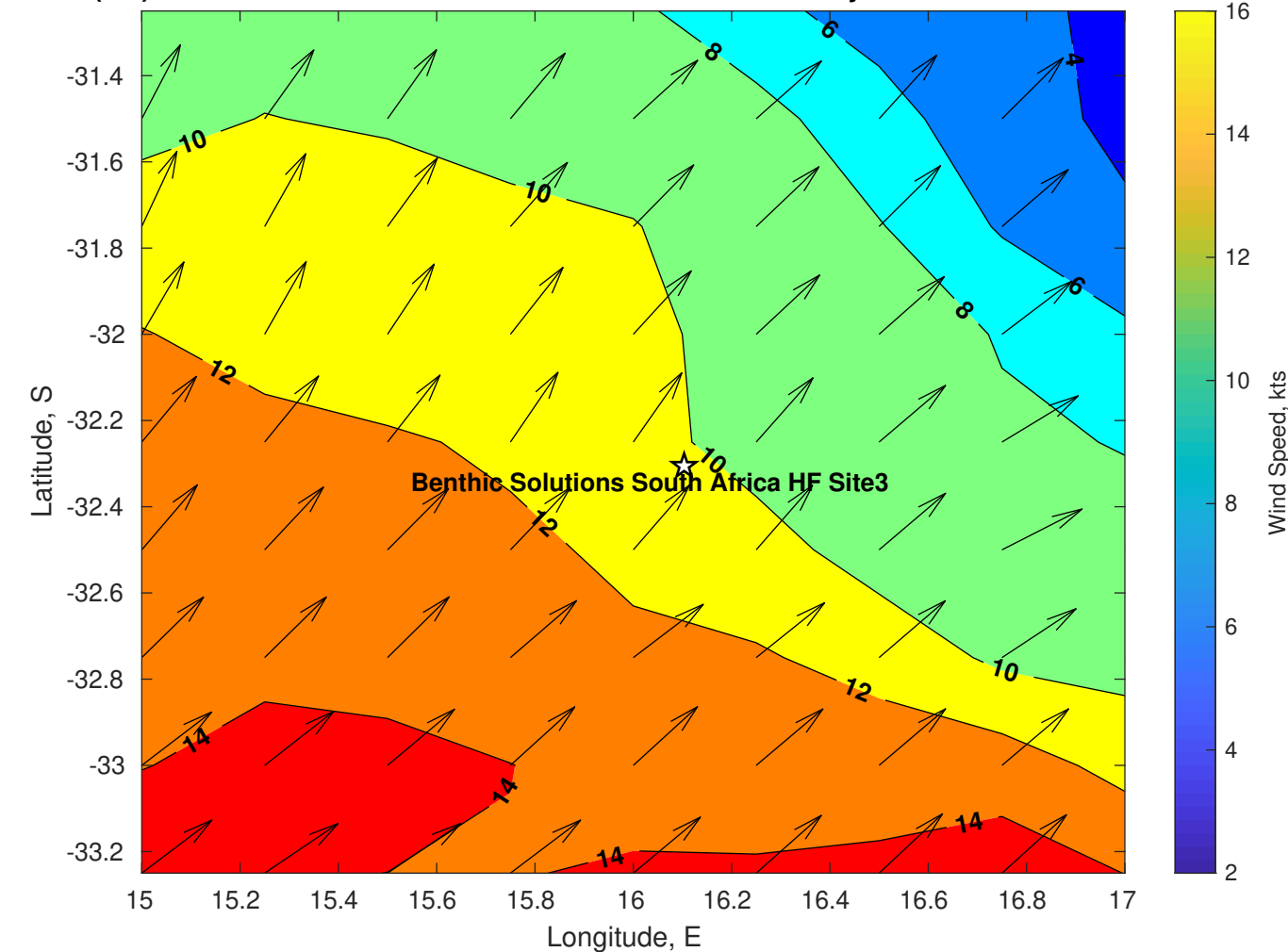
Winds (kts) for Benthic Solutions South Africa HF Site3 at 21-May-2025 09:00:00
