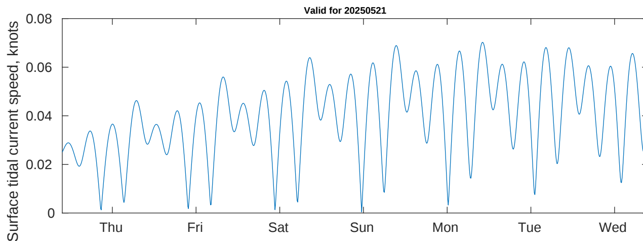
Tidal Currents and Heights for Benthic Solutions South Africa HF Site3 at 20250521
