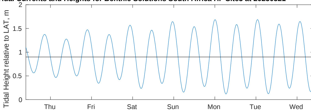
Tidal Currents and Heights for Benthic Solutions South Africa HF Site3 at 20250521
