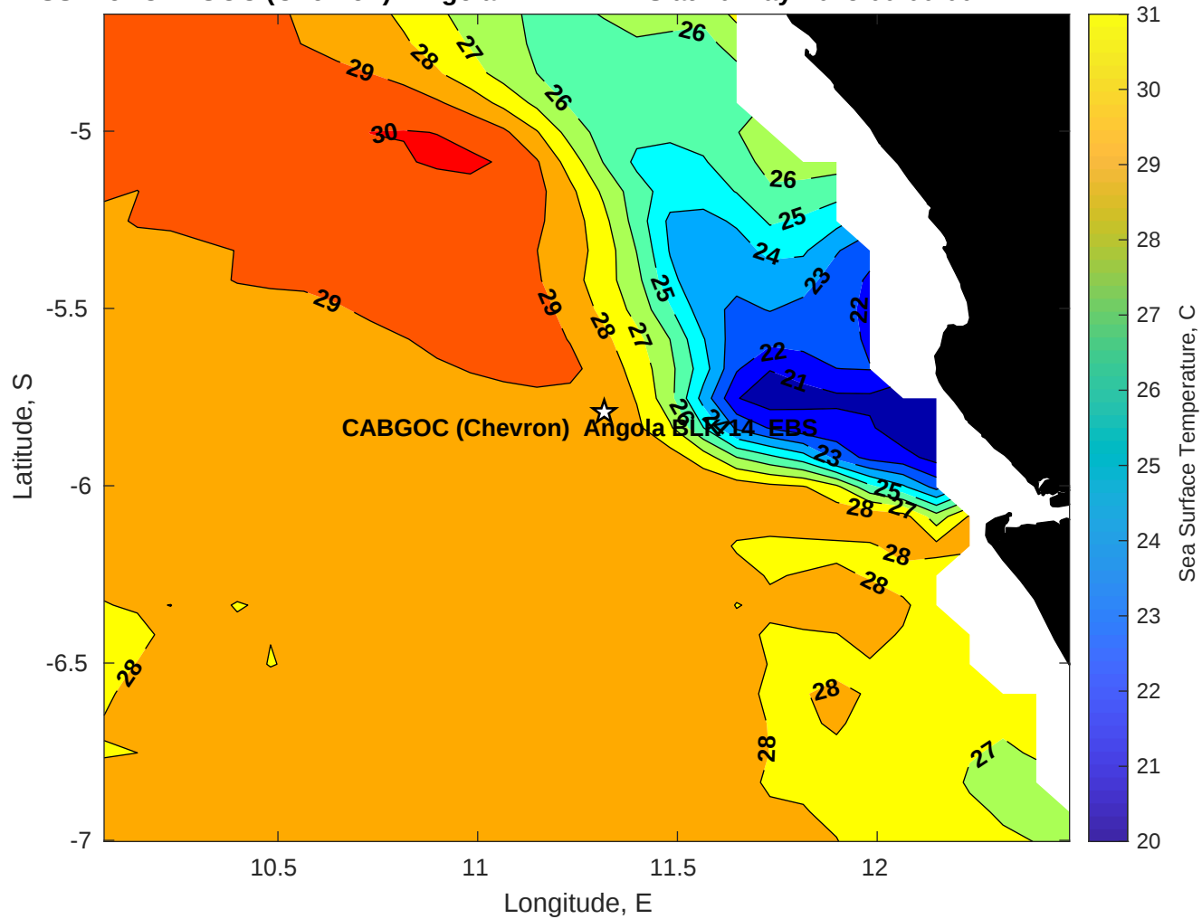
SST for CABGOC (Chevron) Angola BLK 14 EBS at 20-May-2025 00:00:00
