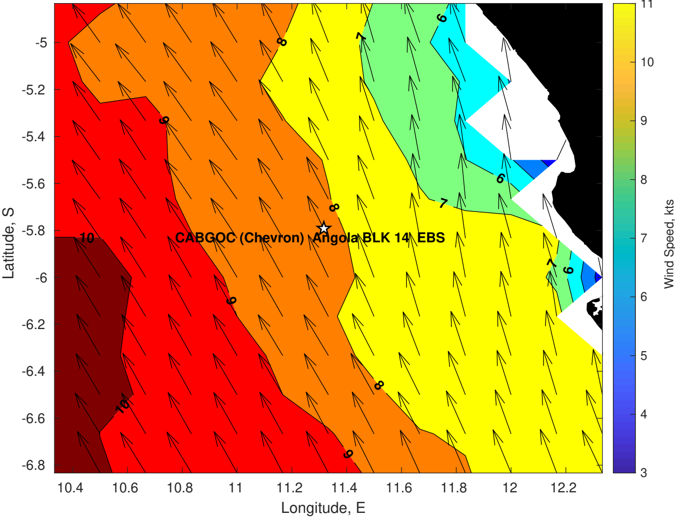
Winds (kts) for CABGOC (Chevron) Angola BLK 14 EBS at 21-May-2025 09:00:00
