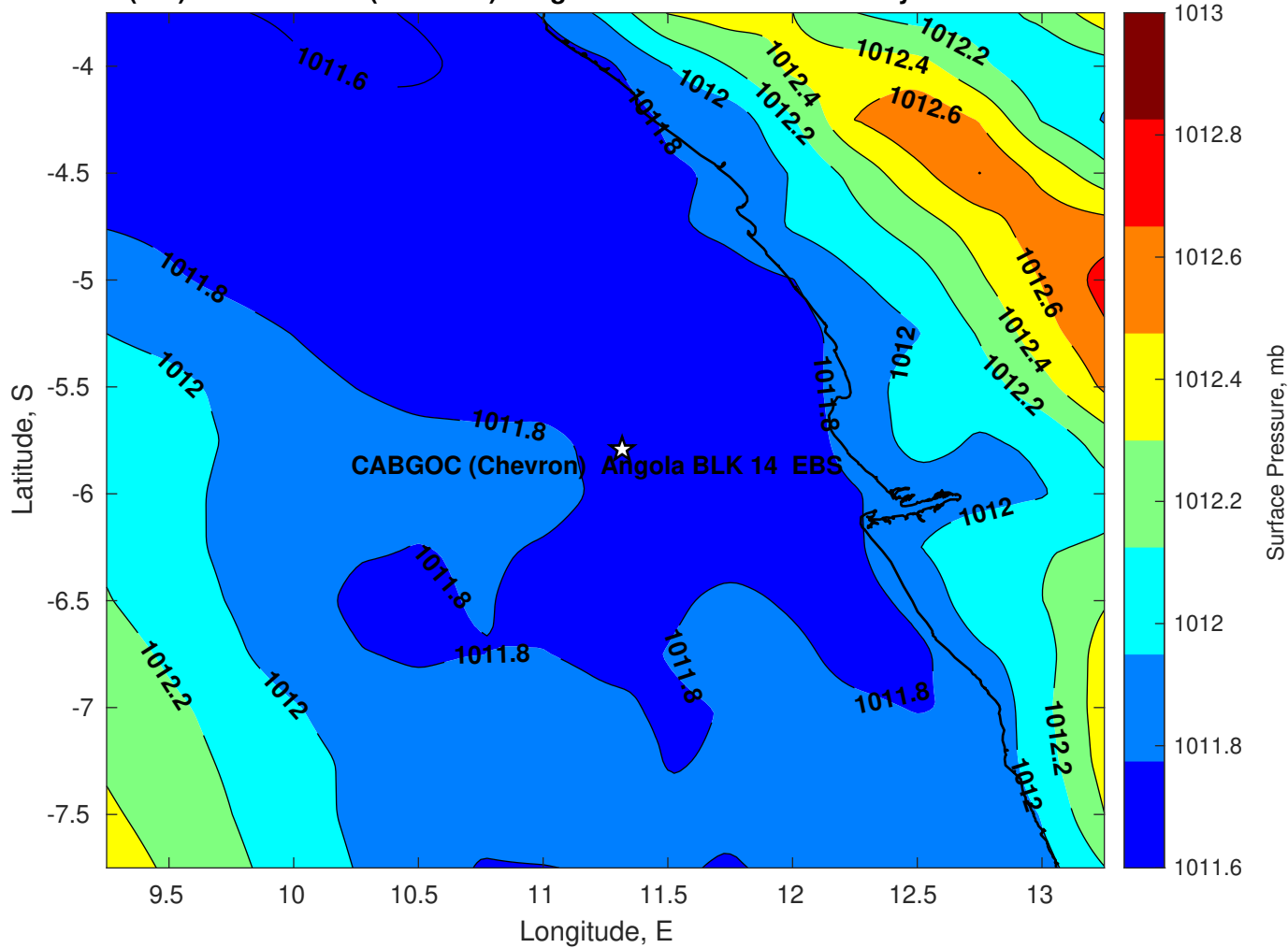
Surface Pressure (mb) for CABGOC (Chevron) Angola BLK 14 EBS at 21-May-2025 00:00:00
