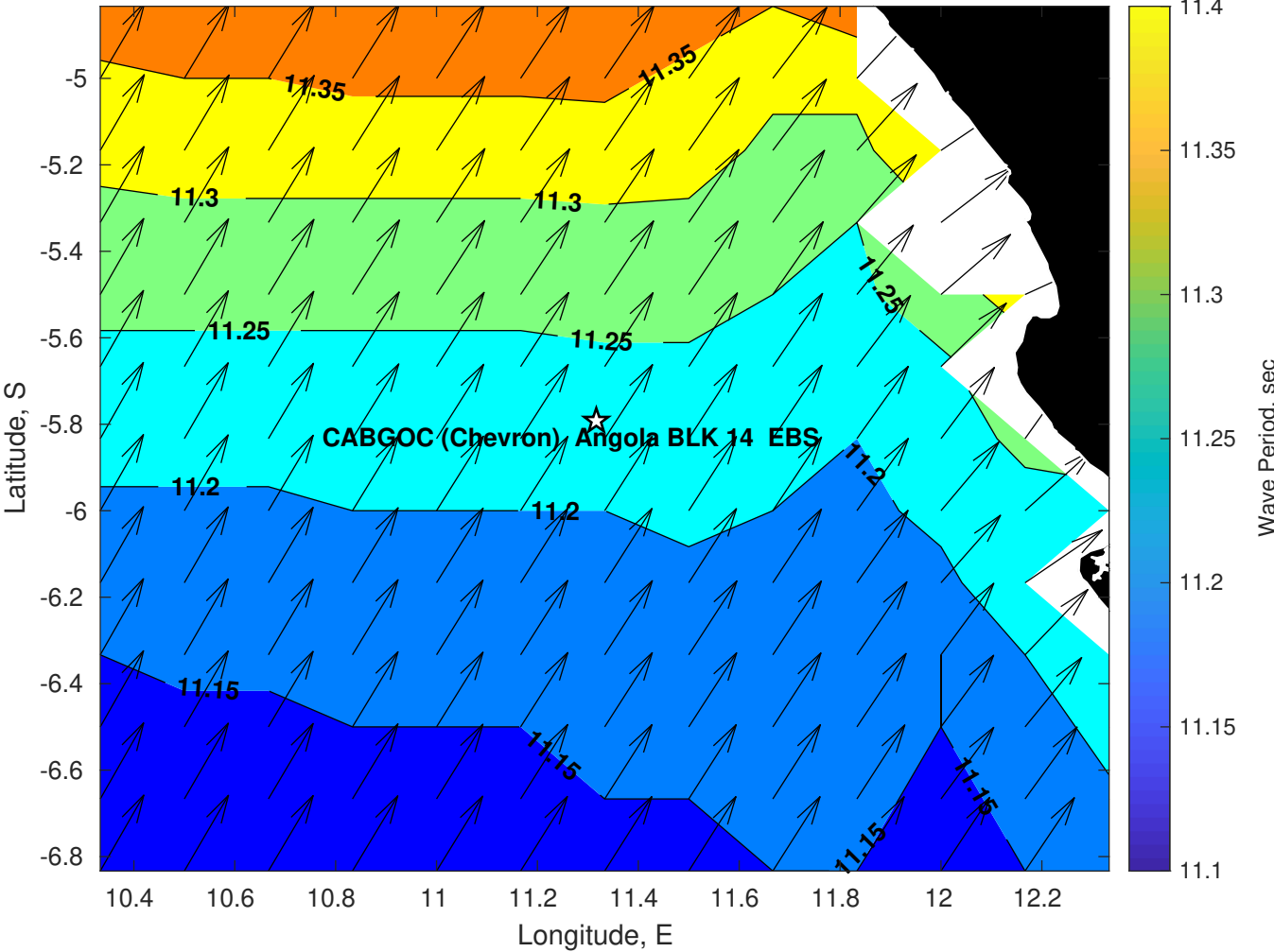
Wave Period (sec) for CABGOC (Chevron) Angola BLK 14 EBS at 21-May-2025 09:00:00
