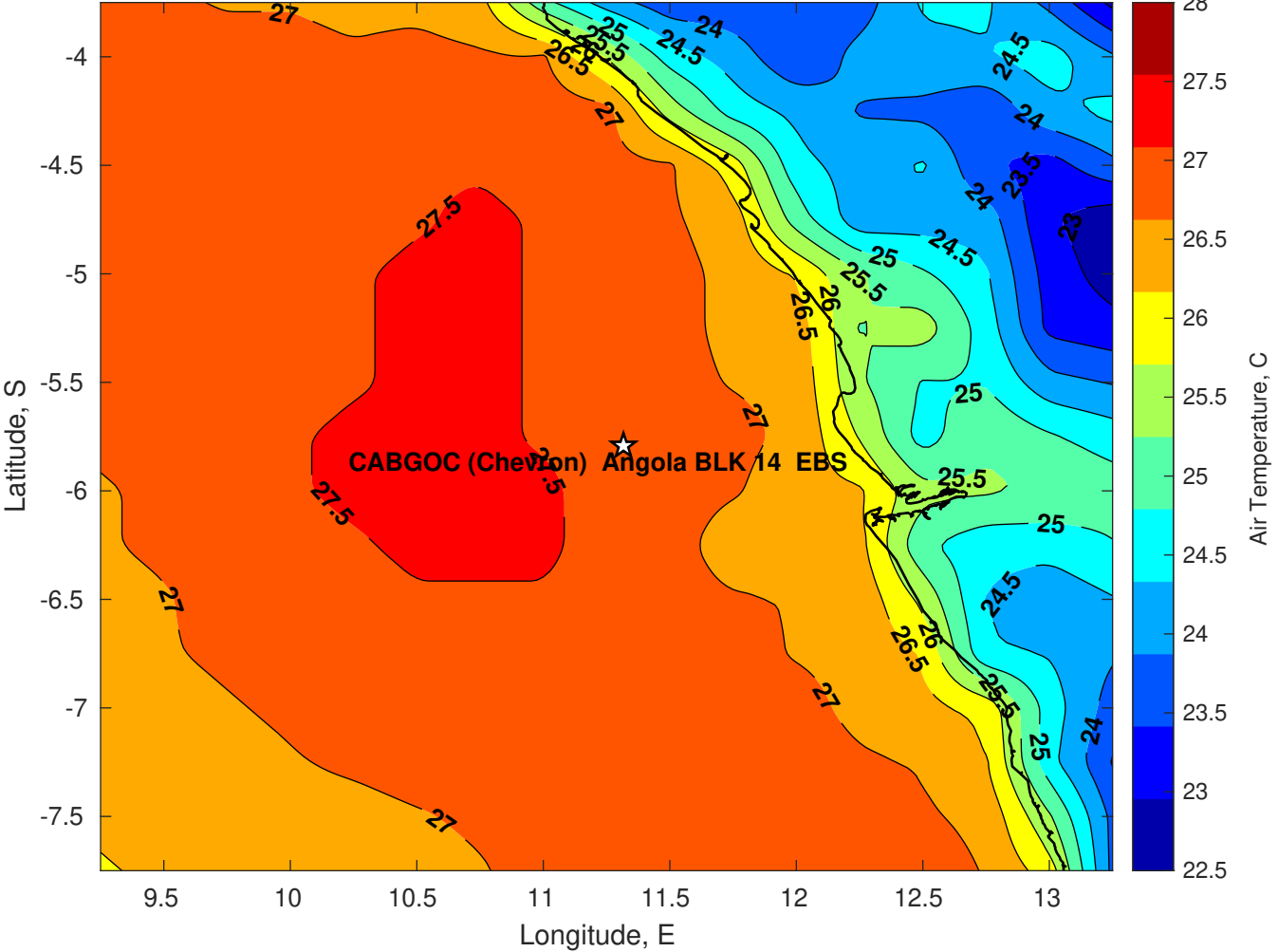
Air Temperature (C) for CABGOC (Chevron) Angola BLK 14 EBS at 21-May-2025
