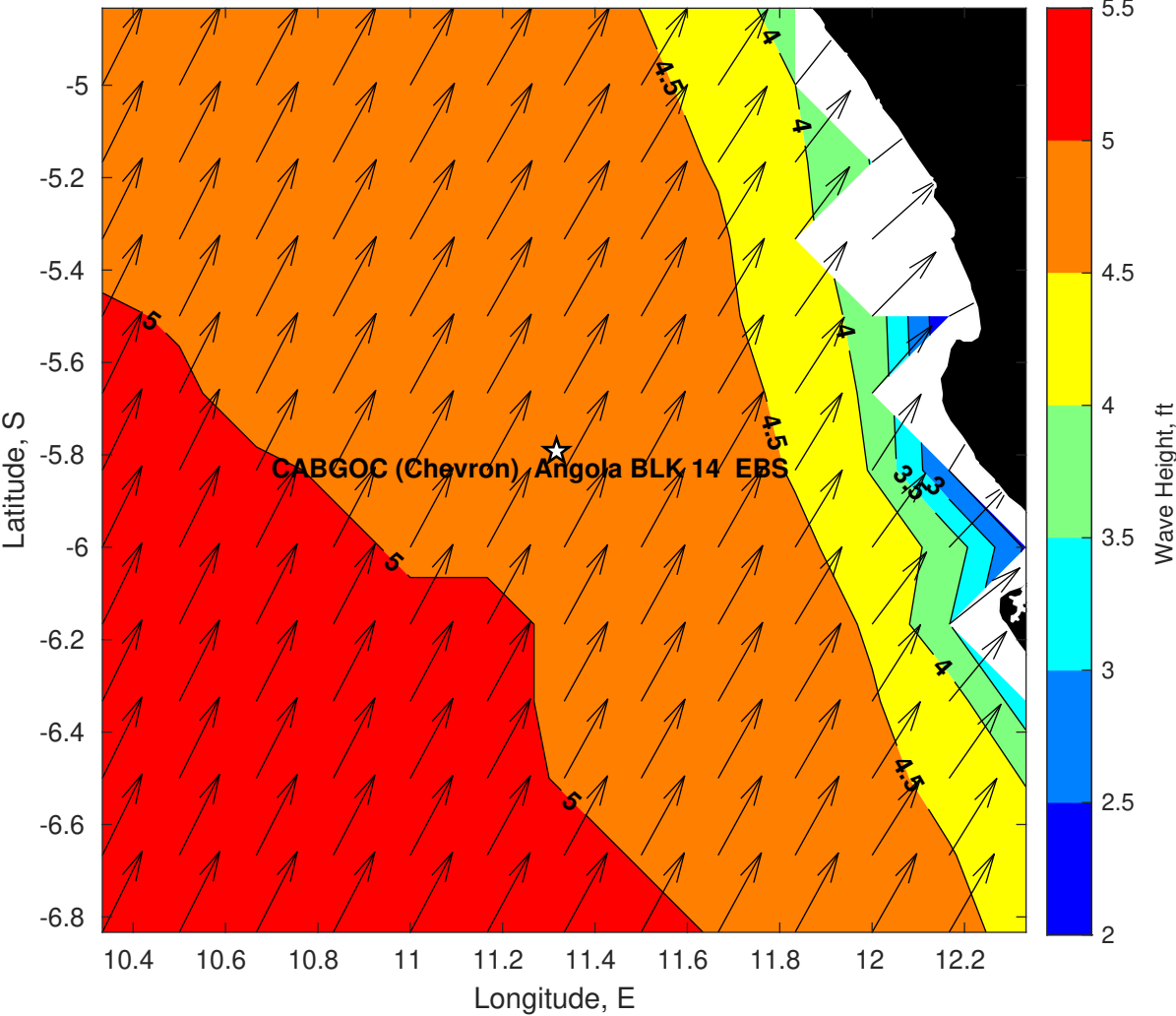
Wave Height (ft) for CABGOC (Chevron) Angola BLK 14 EBS at 21-May-2025 09:00:00
