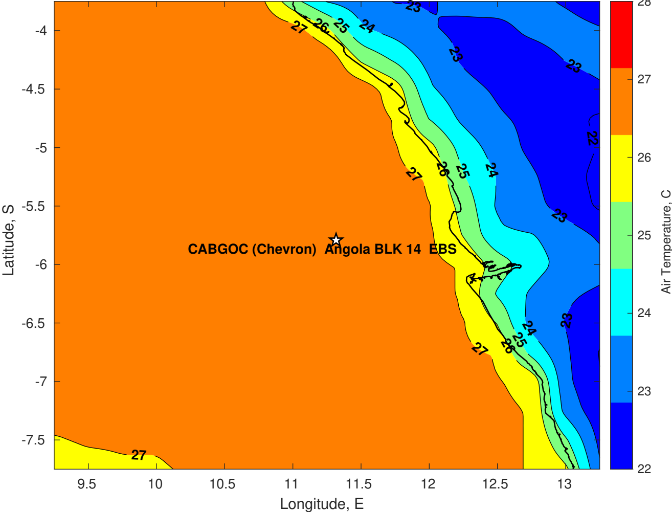
Air Temperature (C) for CABGOC (Chevron) Angola BLK 14 EBS at 21-May-2025
