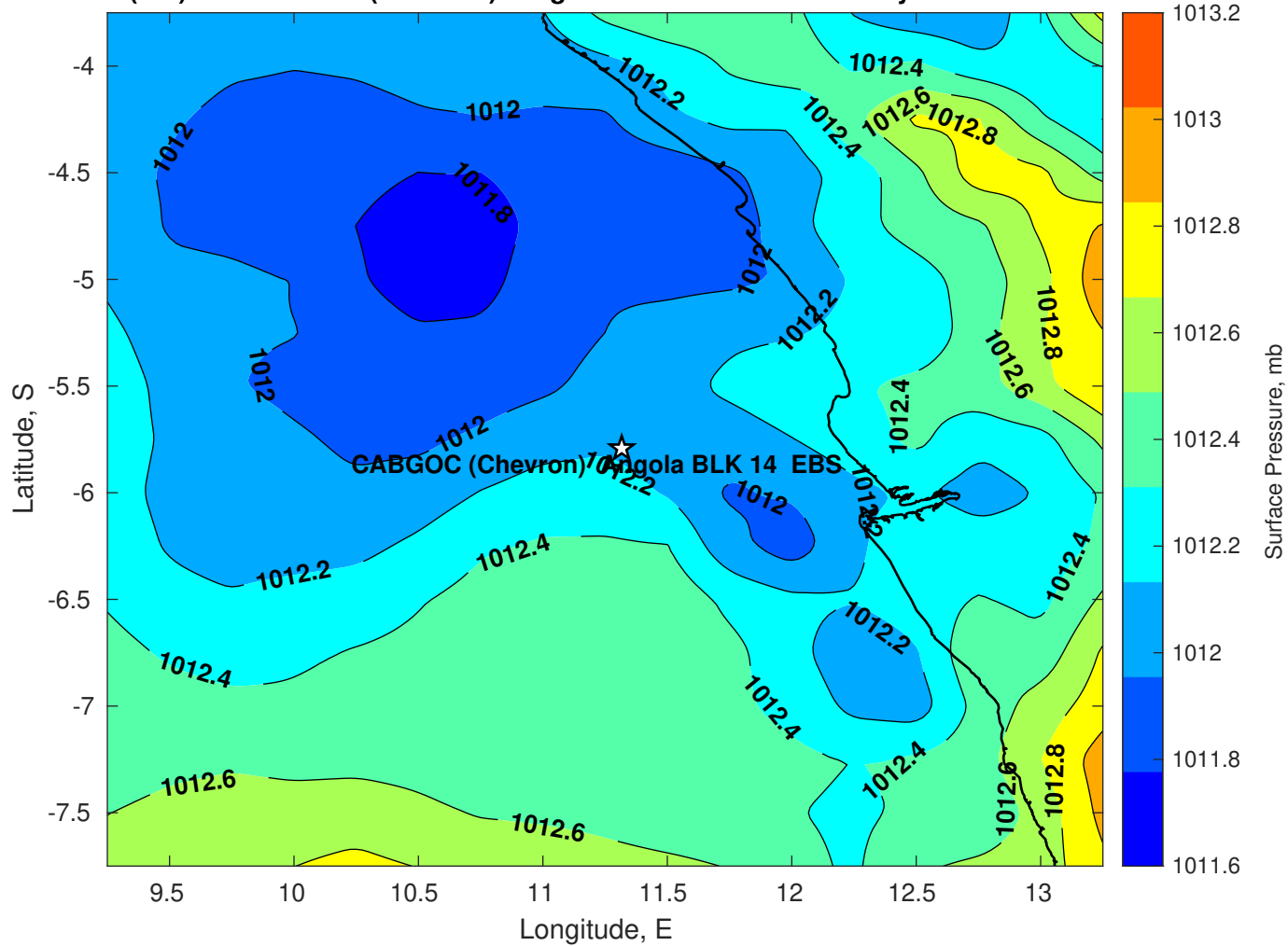
Surface Pressure (mb) for CABGOC (Chevron) Angola BLK 14 EBS at 23-May-2025 00:00:00
