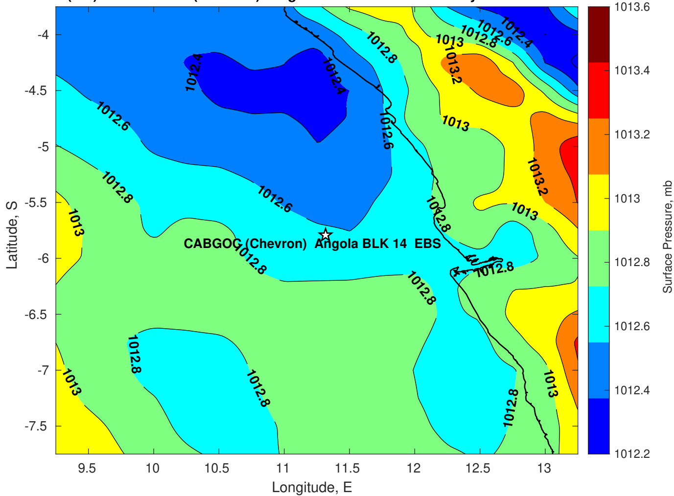
Surface Pressure (mb) for CABGOC (Chevron) Angola BLK 14 EBS at 22-May-2025 00:00:00
