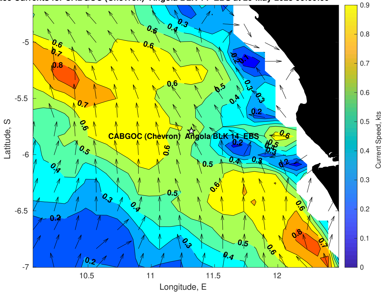
Surface Currents for CABGOC (Chevron) Angola BLK 14 EBS at 20-May-2025 00:00:00
