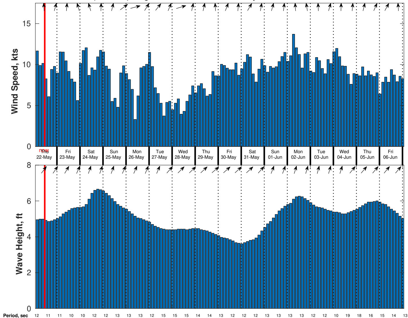
Wind & Wave Forecast for CABGOC (Chevron) Angola BLK 14 EBS from 21-May-2025 02:00:00 to 06-Jun-2025 02:00:00
