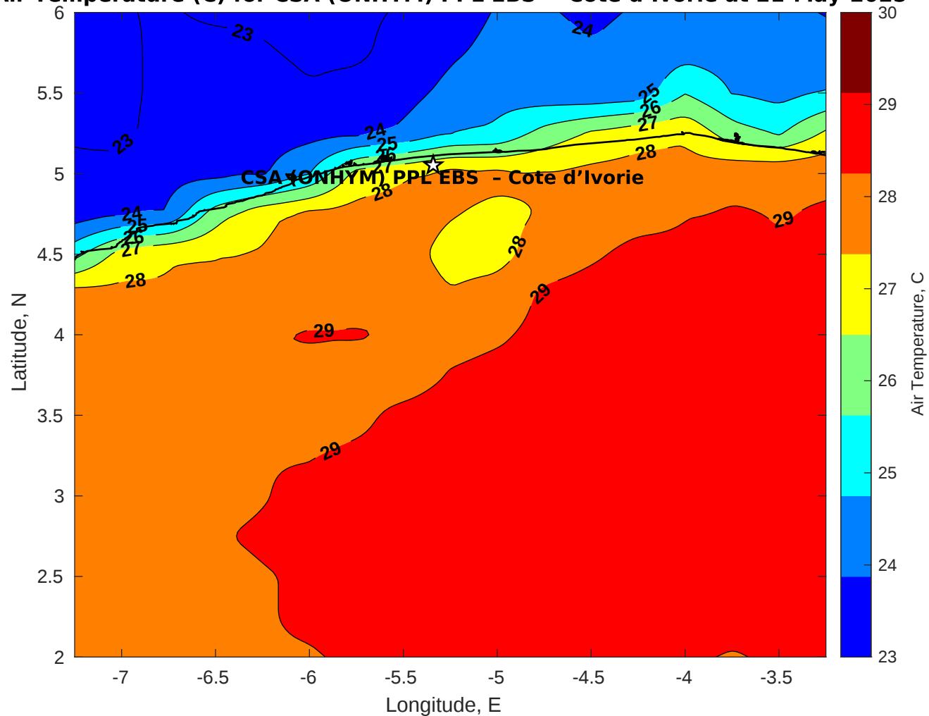
Air Temperature (C) for CSA (ONHYM) PPL EBS - Cote d'Ivoire at 21-May-2025
