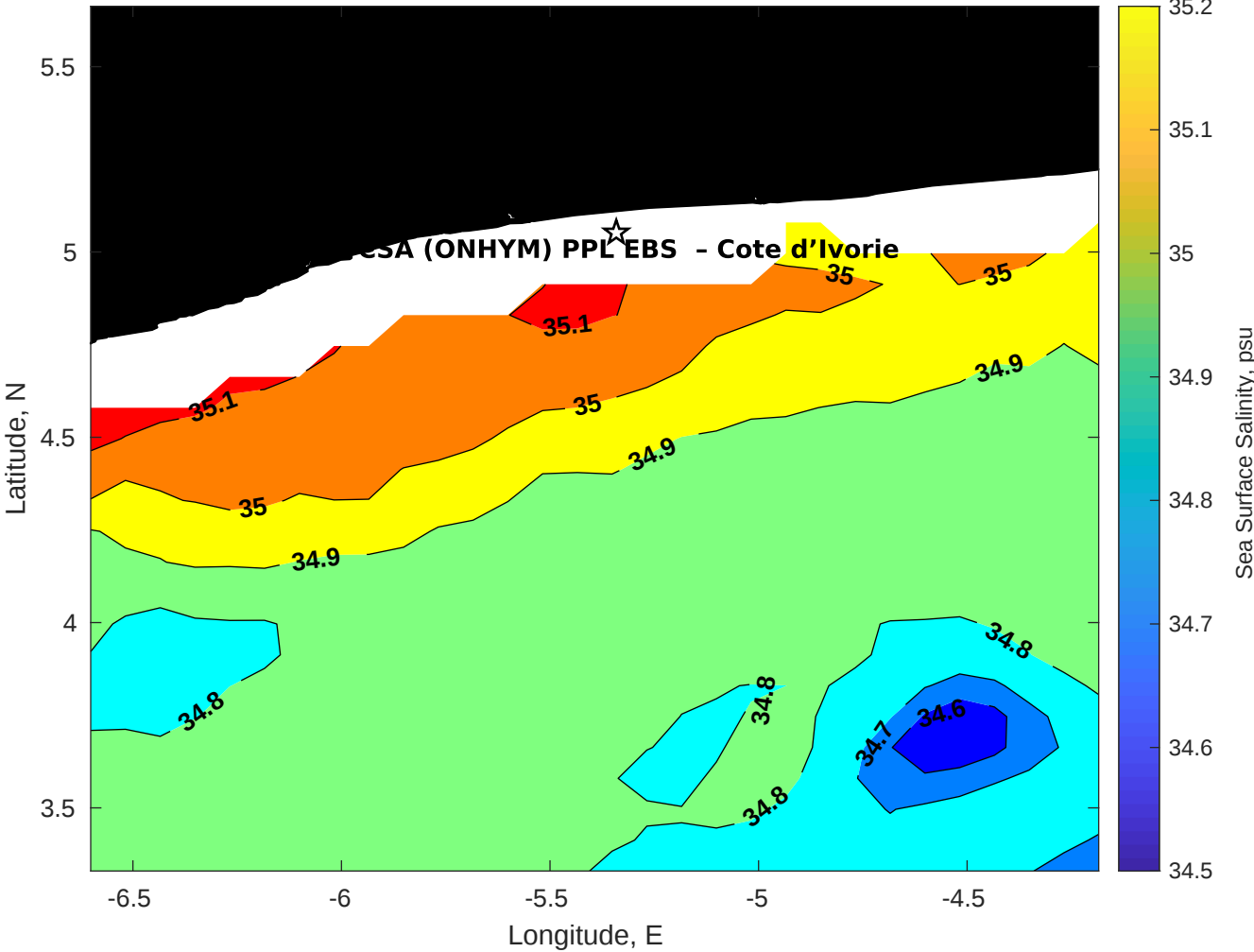
Surface Salinity for CSA (ONHYM) PPL EBS - Cote d'Ivoire at 20-May-2025 00:00:00
