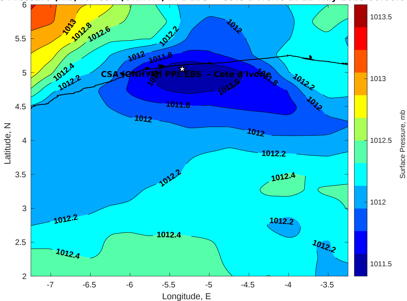
Surface Pressure (mb) for CSA (ONHYM) PPL EBS - Cote d'Ivoire at 21-May-2025 00:00:00
