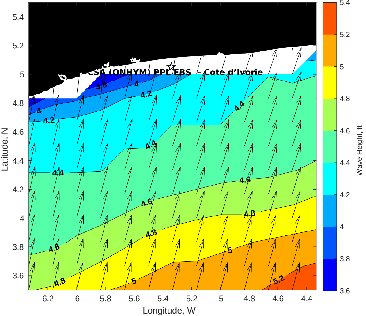
Wave Height (ft) for CSA (ONHYM) PPL EBS - Cote d'Ivoire at 21-May-2025 09:00:00
