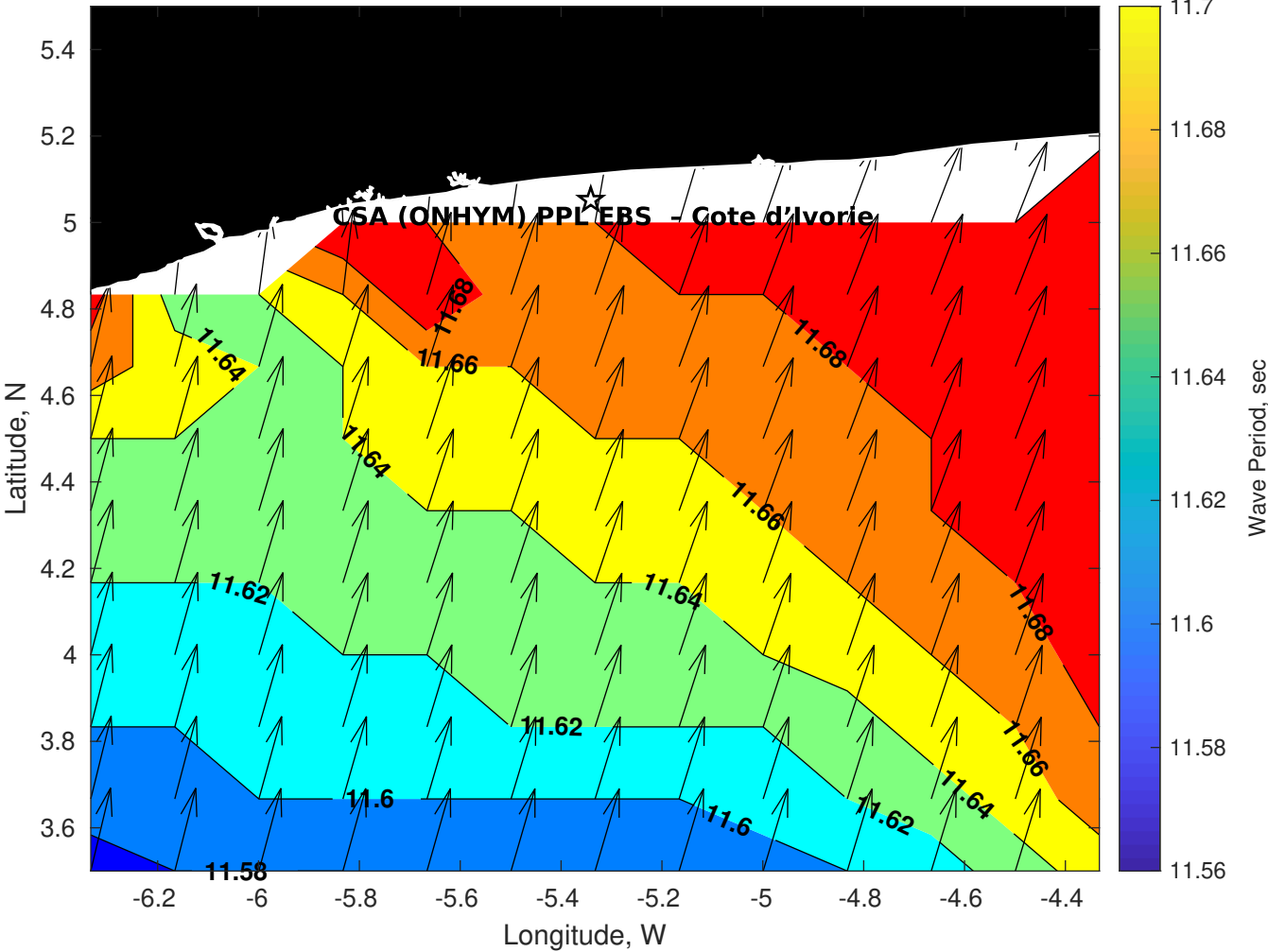
Wave Period (sec) for CSA (ONHYM) PPL EBS - Cote d'Ivoire at 21-May-2025 09:00:00
