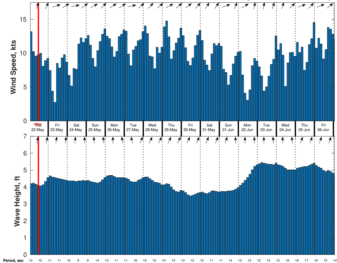
Wind & Wave Forecast for CSA (ONHYM) PPL EBS - Cote d'Ivoire from 21-May-2025 01:00:00 to 06-Jun-2025 01:00:00
