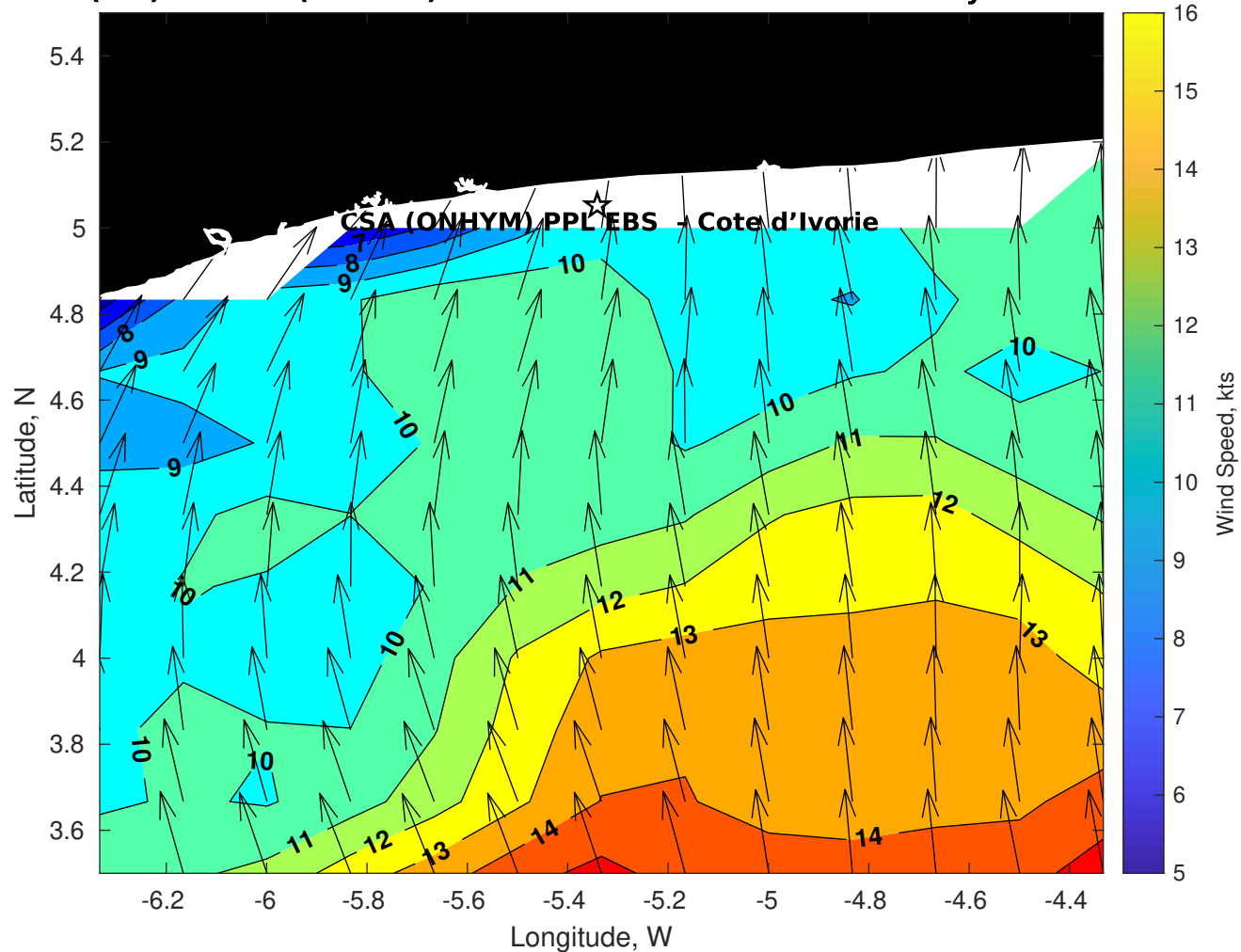
Winds (kts) for CSA (ONHYM) PPL EBS - Cote d'Ivoire at 21-May-2025 09:00:00
