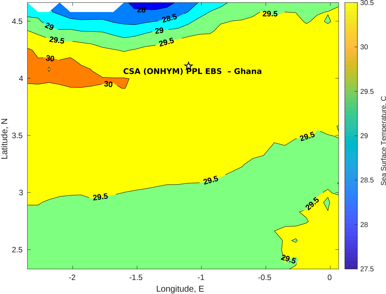
SST for CSA (ONHYM) PPL EBS - Ghana at 20-May-2025 00:00:00
