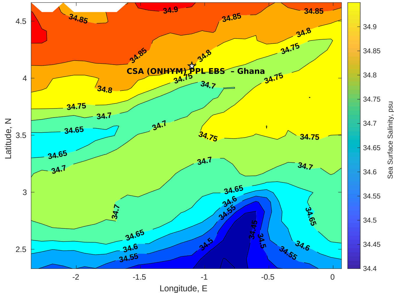
Surface Salinity for CSA (ONHYM) PPL EBS - Ghana at 20-May-2025 00:00:00
