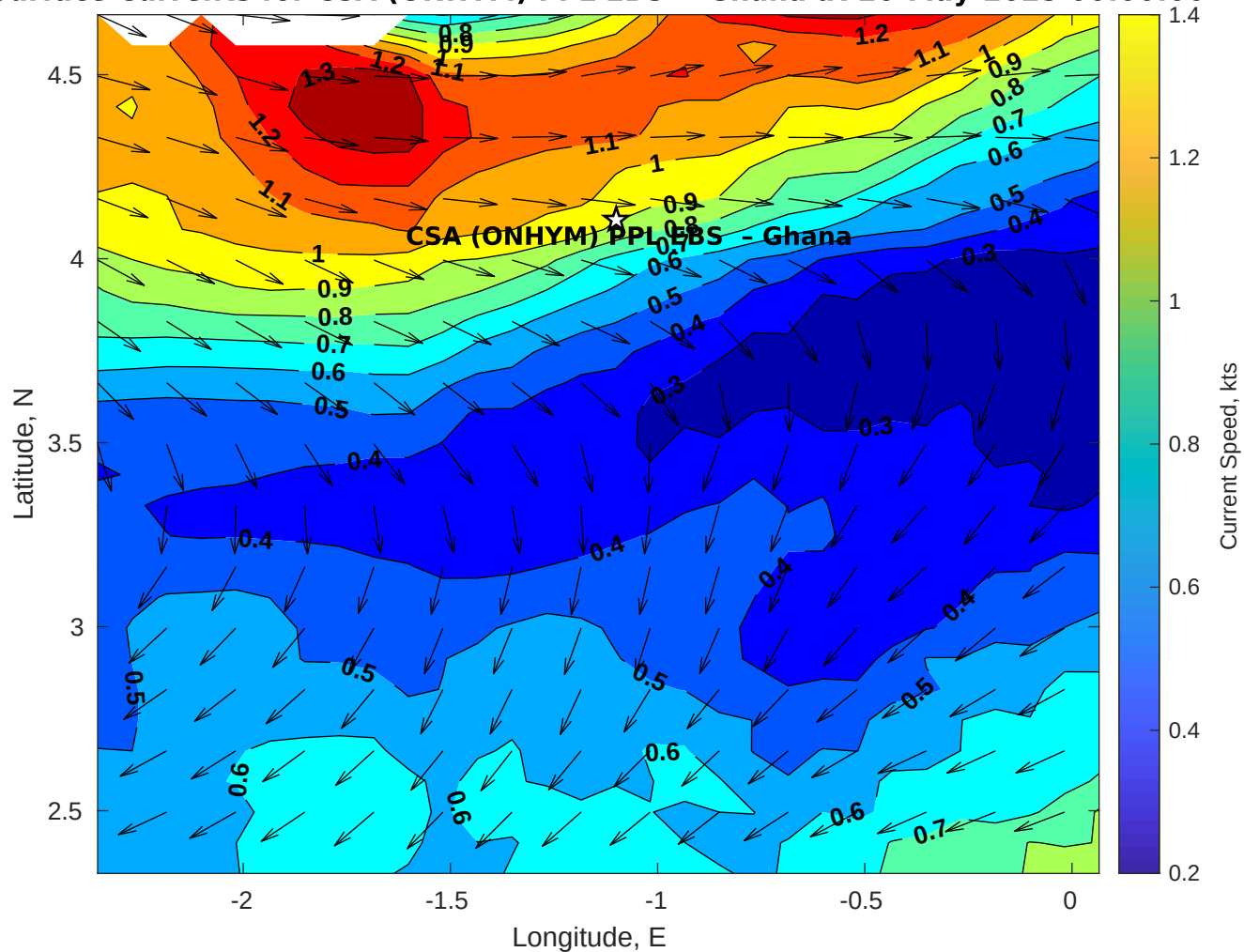
Surface Currents for CSA (ONHYM) PPL EBS - Ghana at 20-May-2025 00:00:00
